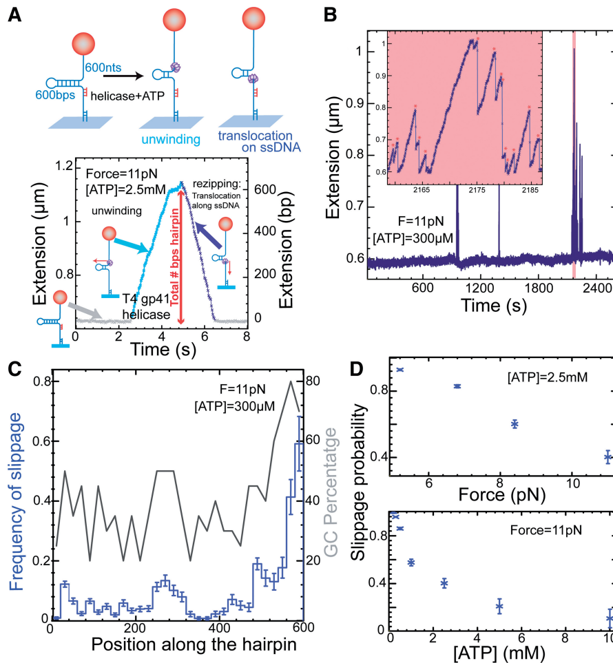
Figure 2. T4 helicase activity on a DNA hairpin substrate. (A) Schematics (upper panel) and experimental trace (lower panel) corresponding to the T4 helicase loaded on the 5' ssDNA tail of the hairpin displaying DNA unwinding activity followed by ssDNA translocation activity concomitant with hairpin reannealing. The measured extension change (left axis) is converted to the number of base pairs unwound (right axis) by assigning the full length of the hairpin to the maximum number of unwinding events. (B) Bursts of helicase activity were observed every tens of minutes ensuring the monitoring of a single helicase complex (10–20 nM gp41 and 300 μM ATP). Inset: Enlargement of the experimental trace exhibiting repeated cycles of unwinding and slippage (red asterisk). (C) The frequency of helicase slippage events (blue) correlated with the percent GC content of the substrate (grey) when plotted against the corresponding position of the DNA substrate. The error bars are proportional to the inverse of the square root of the number of points for each individual bin. The number of molecules and enzymatic traces analysed is N_{\text{mol}} = 9 and N = 288 , respectively. (D) The percentage of experimental traces which exhibited helicase slippage events as a function of the applied force (upper panel) and the ATP concentration (lower panel) are shown. Error bars are the SEM. The number of molecules and enzymatic traces analysed varies between N_{\text{mol}} = 17\text{--}42 and N = 163\text{--}489 , respectively, depending on the force and ATP condition.
