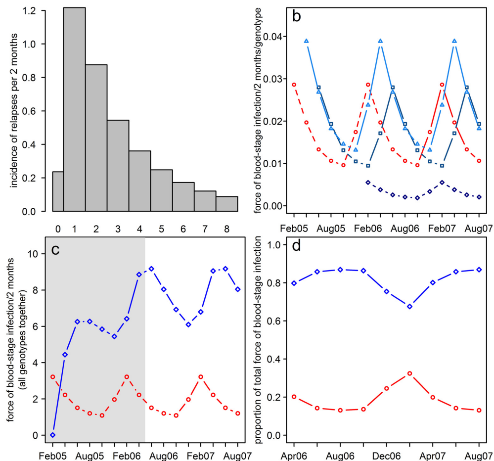
Fig 3. Predicted P. vivax relapse and primary infection for a three-year-old girl. (a) Estimated incidence of relapse per infection by two month interval from the primary infection. (b) Estimated incidence of primary infection and of relapses subsequent to primary infections one, two and six intervals earlier. Red circles: The incidence of primary infections prior to (dotted line) and during (solid line) the study period. Blue lines: The incidence of relapses subsequent to primary infections occurring one (light blue triangles), two (mid-blue squares) and six (dark blue diamonds) intervals earlier. (c) Estimated force of blood-stage infection from primary infections and relapses. Red circles: primary infections, blue diamonds: relapses. Shaded area is the warm-up period prior to the study, unshaded area is the study period itself. (d) Estimated proportion of the force of blood-stage infection from primary infections and relapses during the study period. Red triangles: primary infections, blue diamonds: relapses. The predictions are for a three-year old girl in Ilaita village with no ITN use using the results for MS16.
