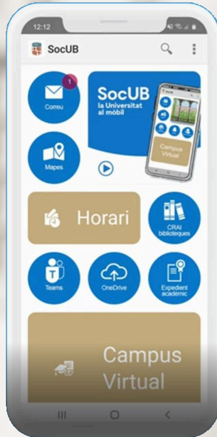
SocUB App
