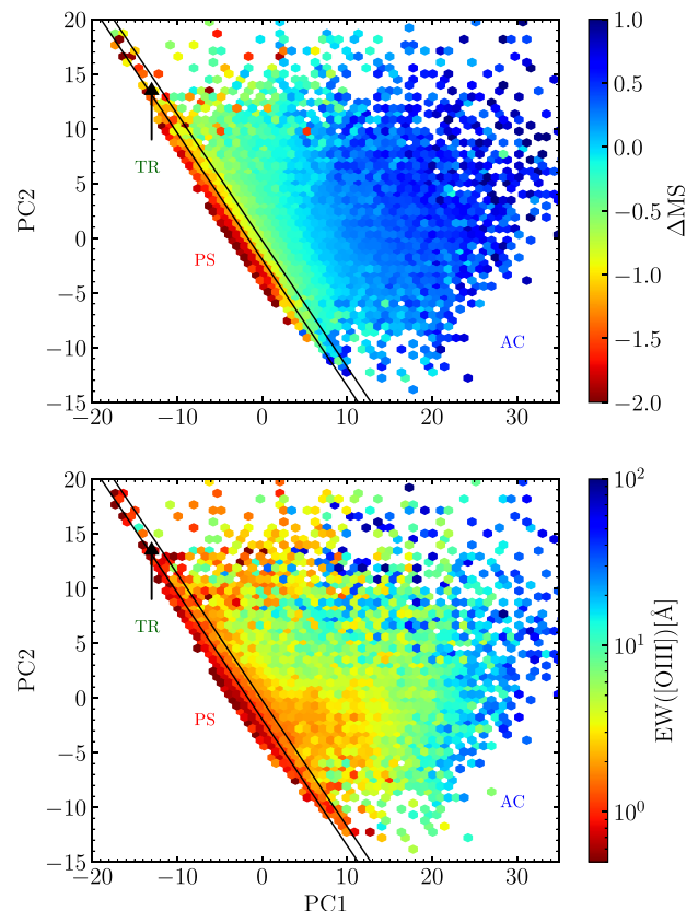
Figure 2. Alternative versions of the PC1–PC2 diagram for our core sample of nearby S0 galaxies. The scatter plots include a colour code that varies according to the mean value of \Delta MS (equation (3); top ) and the [O \text{ III}]\lambda 5007 \text{ \AA} EW ( bottom ) in each of the hexagonal cells in which the data has been grouped. Two parallel black straight lines show the best linear approximations to the PS/TR and TR/AC dividers. Note that the number of measurements used to build both plots is not exactly the same, since the data in the bottom panel obey the additional constraint AoN[O \text{ III}] > 1.5 (see text).
