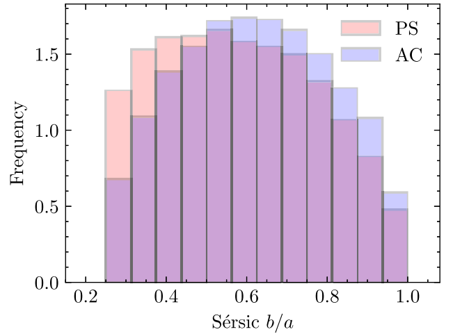
Figure 13. Observed distribution of inclinations for the two main spectral subpopulations of lenticulars in the MLSS0.
