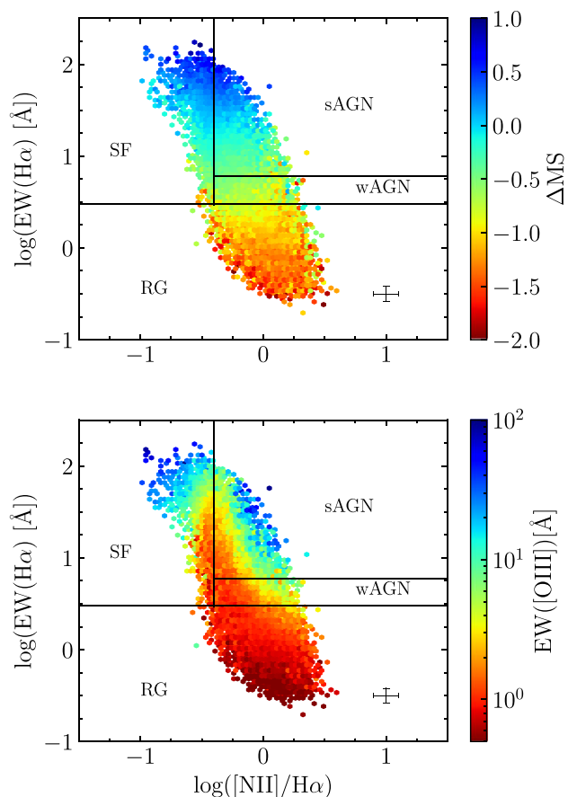
Figure 6. Same as in Fig. 2, but for the WHAN diagram. The horizontal black solid line at \text{EW}(\text{H}\alpha) = 6 \text{ \AA} represents the optimal transposition of the Kewley et al. (2006) divider between sAGN and LINER derived in Cid Fernandes et al. (2010). A second horizontal division line at \text{EW}(\text{H}\alpha) = 3 \text{ \AA} separates the LINER zone into wAGN and RG (see text), while the vertical black solid line at \log([\text{NII}]/\text{H}\alpha) = -0.4 mimics the divider between SF galaxies (on the left) and all AGNs (on the right) of Stasińska et al. (2006). The error bars in the bottom-right corners of the panels show the medians of the errors in both axes.
