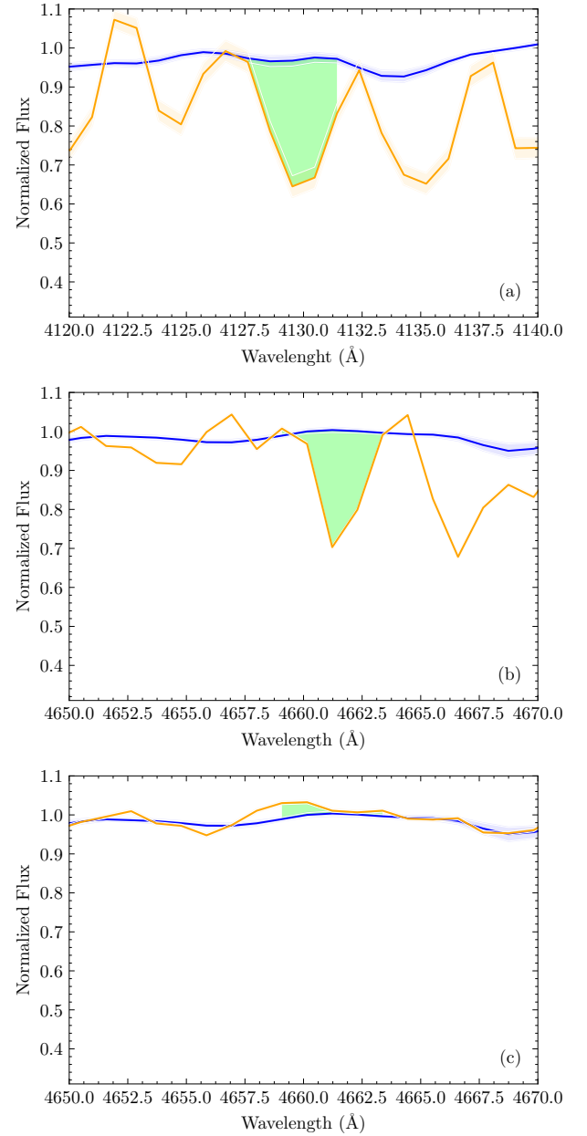
Fig. 2. Comparison of certain observed lines in F5 stars (orange curves) with average flux inferred from whole spectral class (blue curves). The lighter bands surrounding the fluxes show their associated uncertainties, while the green colored areas identify the integrated flux differences that we attribute to lines from Eu. Panel a : F5 star (specobjID=3719984370237415424) that shows a substantial flux deficit compared to the mean in the 4127–4131 Å wavelength range that encompasses an important line of Eu II (see Table 1). Panel b : another F5 star (specobjID=2786716958031191040) also showing a significant flux deficiency in the 4659–4663 Å range, which is the interval of wavelengths where one expects to find a strong Eu I line. In both cases the stars have been identified as positive detections. In contrast, panel c shows a third F5 star (specobjID=3002850987342928896) that does not show evidence for the existence of this latter line in absorption, which classifies it as a non-detection.
