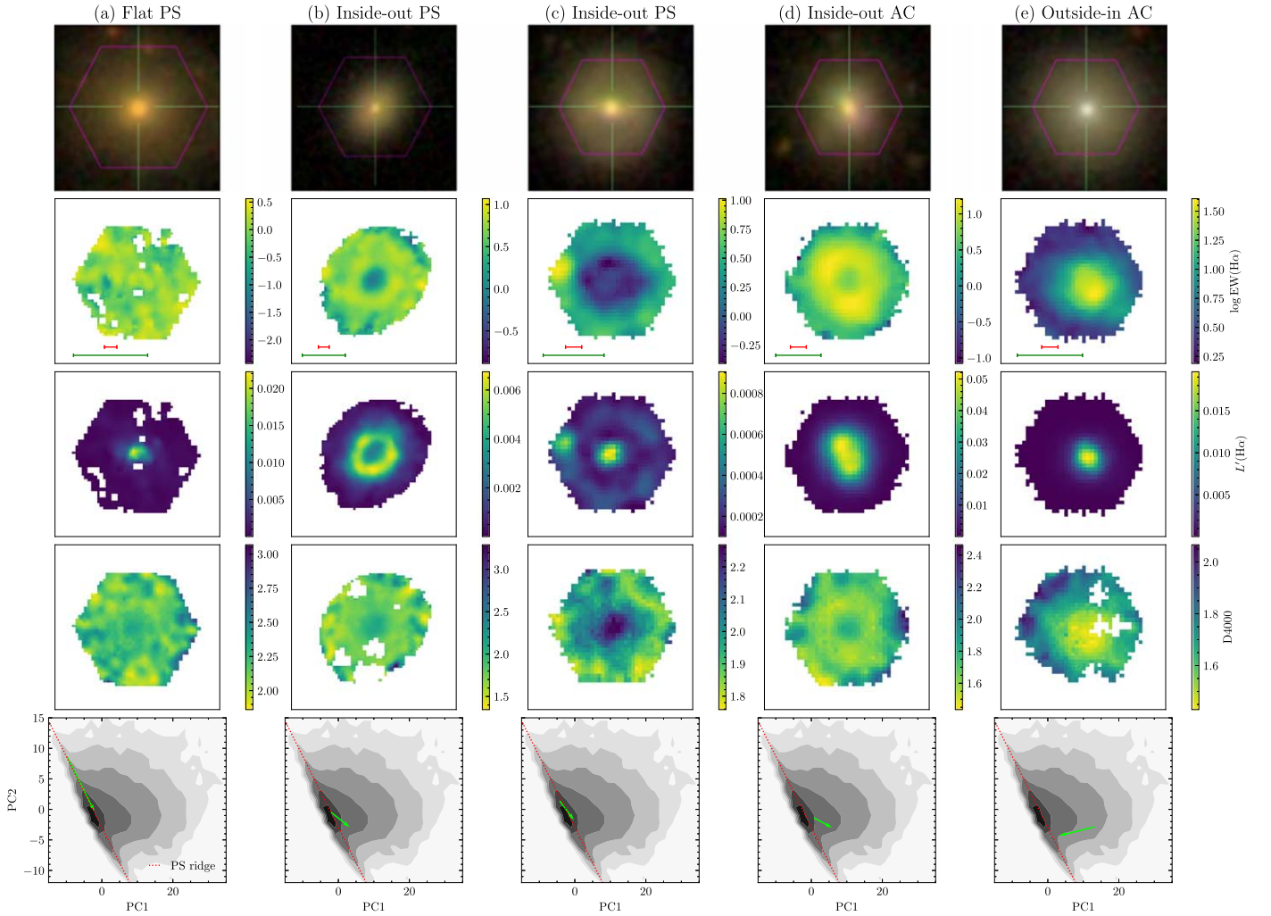
Figure 3. Examples of spectral maps and spectral profiles of S0 galaxies. The second, third, and fourth rows show, in this order, maps of the EW(H \alpha ), L'(\text{H}\alpha) , and D4000 spectral indices. Only spaxels with all quality flags equal to zero are drawn. The green and red horizontal lines included in the EW(H \alpha ) panels indicate, respectively, the galaxies’ Petrosian half-light diameter in the r band and 2\sigma_{\text{PSF}} . The bottom row shows the vectorized spectral profiles of the galaxies in the PC1–PC2 subspace. The true color images of the galaxies are shown in the first row, with the overlapping violet hexagonal frames depicting the footprint of MaNGA’s bundles (images’ source: https://data.sdss.org/sas/dr15/manga/ ). Galaxies in columns (b), (c), and (d) show clear rings in EW(H \alpha ) (i.e., they have ring scores r \geq 6 ), whereas no rings are observed for the galaxies in columns (a) and (e) ( r < 3 ).
