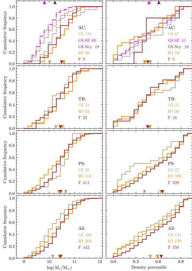
Figure 8. Left panels: cumulative distribution functions of M_* for the different types of activity profiles of the MaNGA S0 galaxies. The solid lines show outside in (OI, light brown), inside out (IO, orange) and flat (F, brown) gradients. Each panel depicts the CDFs segregated by activity class, from top to bottom: active cloud (AC), further divided into galaxies with a SF (dash-dotted line) and Seyfert (dotted line) status assigned by Thomas et al. (2013) , transition region (TR), and passive sequence (PS), respectively, while the bottom panel shows aggregate results. The filled triangles indicate the medians of each CDF. The size of each subset is shown in the legend next to the profile labels. Right panels: as the panels on the left, but using as random variable the percentile corresponding to the local density of the environment (see Section 2).
