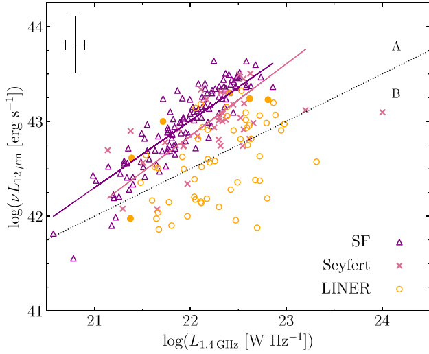
Figure 11. Observed mid-IR 12\mu\text{m} luminosity versus monochromatic 1.4 GHz radio luminosity for the main BPT types of nearby S0 galaxies, SF (purple empty triangles), Seyfert (pink crosses) and LINER (orange empty circles), simultaneously detected in the SDSS, WISE and FIRST surveys. Filled symbols are used for the six LINERs that are also X-ray emitters. The dotted line, which divides the diagram in two sectors (letters A and B), is the same as in fig. 3 of Rosario et al. (2013). Also following these authors, we have used an ordinary-least-squares bisector algorithm to estimate the linear regression lines for the SF (purple line) and Seyferts on sector A (pink line). These lines are included in the plot for the sole purpose of allowing the mean trends of both subsets of objects to be compared at a glance. The error bars in the upper-left corner show the typical 1\sigma uncertainties of the data for both axes.
