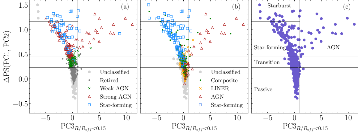
Figure 2: Distribution of 937 S0s in the \Delta\text{PS} -PC3 diagram classified using the WHAN (a), the BPT (b), and the PCA (c) schemes. The two lower horizontal lines correspond to the PS/TR/AC class dividers derived in Jiménez-Palau et al. (2022b), while the vertical line has been introduced to distinguish the regions where galaxies cluster depending on whether the dominant ionization source is star formation or AGN. The upper-left corner contains galaxies with strong emission lines ( \text{EW}(\text{H}\alpha) \geq 100 \text{ \AA} ) likely associated with a starburst. Note the segregation of the WHAN classes: retired, weak AGN and strong AGN/star-forming along \Delta\text{PS} (a); and the BPT classes: star-forming/LINER and AGN along PC3 (b).
