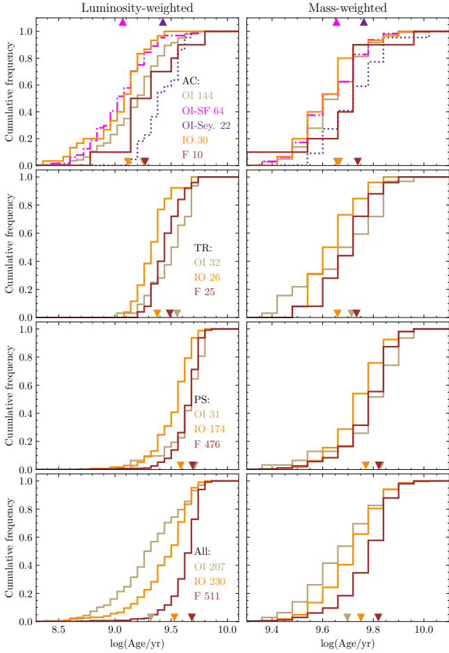
Figure 9. As Fig. 8 but using as random variables the luminosity-weighted age (left panels) and mass-weighted age (right panels) of the stellar populations.
