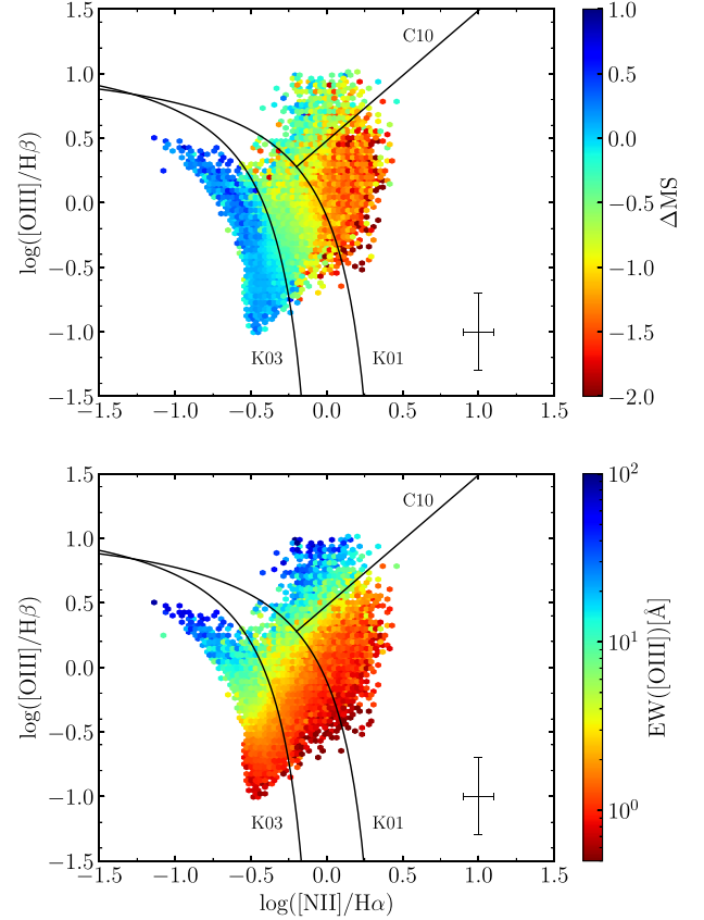
Figure 5. Same as in Fig. 2 but for the BPT–NII diagram. Black curves show the demarcation lines listed in Table 1. As in Fig. 4, we only plot galaxies whose parameters pass our quality filters. The error bars in the bottom-right corners of the panels show the medians of the errors in both axes.
