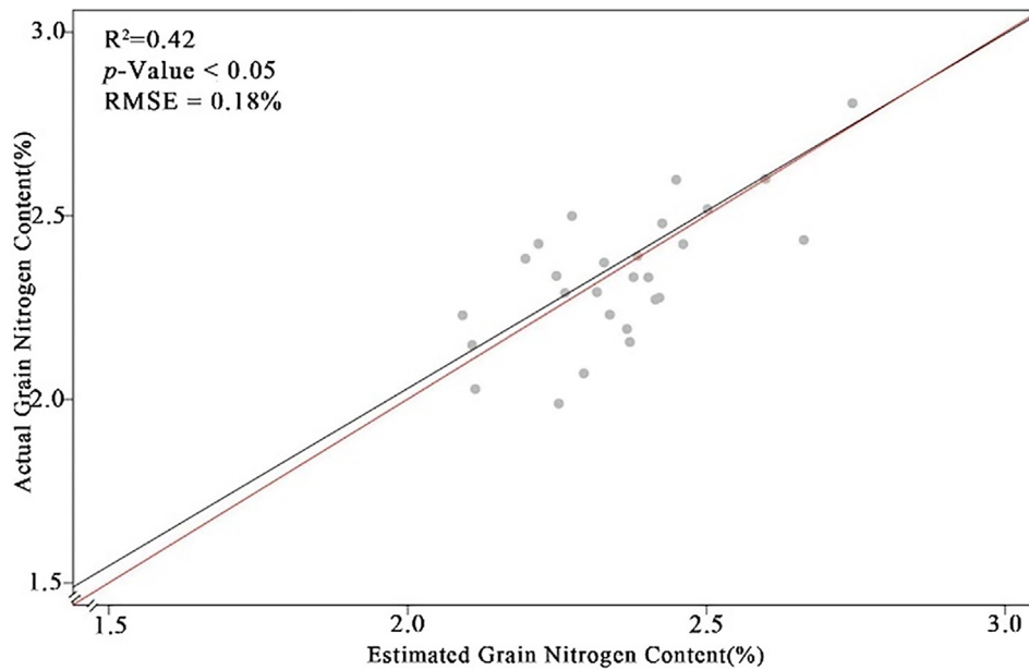
Fig. 6 – Validation of the stepwise multilinear regression models for UAV multilinear data at anthesis as the most suitable model for GNC estimation, 30% of the data set of the experimental plots were used for validation. The equation of the model is shown in Table 5. The R^2 , p -value and root mean square (RMSE) are shown. The red line indicates 1:1.
