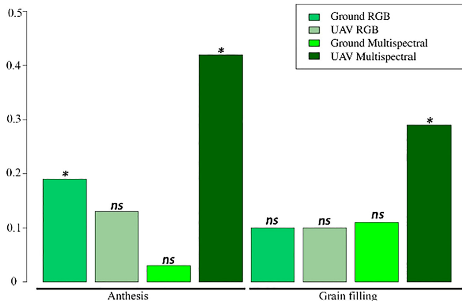
Fig. 5 – Summary of the obtained R^2 at validation for GNC estimation with RGB and multispectral sensors at ground and aerial levels, the * indicates a significance of p -value < 0.05 while ns refers to no significance. The two phenological stages studied are shown (anthesis and grain filling).
