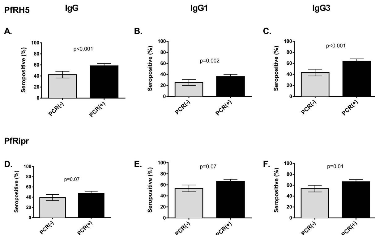
Figure 3. Seroprevalence of total IgG and subclass response to PfRH5 and PfRipr by concurrent parasitemia measured by PCR. Results are shown as percentage seropositive, as determined by ELISA. Error bars indicate standard error of proportion (SE). Results are shown by parasitemic status at enrolment (PCR(–) or PCR(+)). Top row: PfRH5 Bottom row: PfRipr. Results are shown for (A)/(D) Total IgG, (B)/(E) IgG1 and (C)/(F) IgG3 left to right. P values indicate chi square test.
