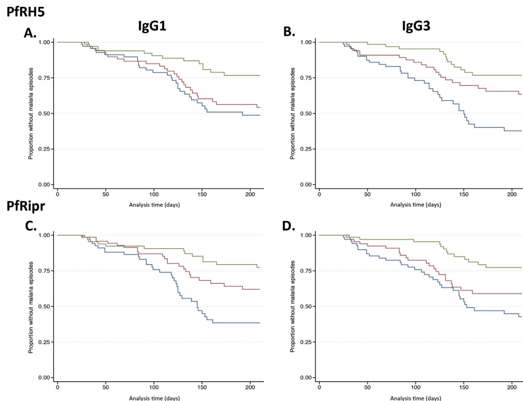
Figure 4. Risk of symptomatic P. falciparum episode during follow-up relative to IgG1 and IgG3 to PfRH5. Kaplan-Meier curves show the proportion of children that remained free of malaria episodes over time for IgG subclass responses against PfRH5 and PfRipr (A) IgG1 to PfRH5; (B) IgG3 to PfRH5; (C) IgG1 to PfRipr; (D) IgG3 to PfRipr. Antibody responses were divided into 3 equal response groups: high (green line), medium (red line), and low (blue line) antibody reactivity. Unadjusted data are shown. Wilcoxon log rank tests were carried out: (A) p = 0.004 ; (B) p < 0.001 ; (C) p < 0.001 ; (D) p < 0.001 . Symptomatic P. falciparum infection was defined as fever ( >37^{\circ}\text{C} ) plus a parasite load of 5000 parasites/ \mu\text{L} .
