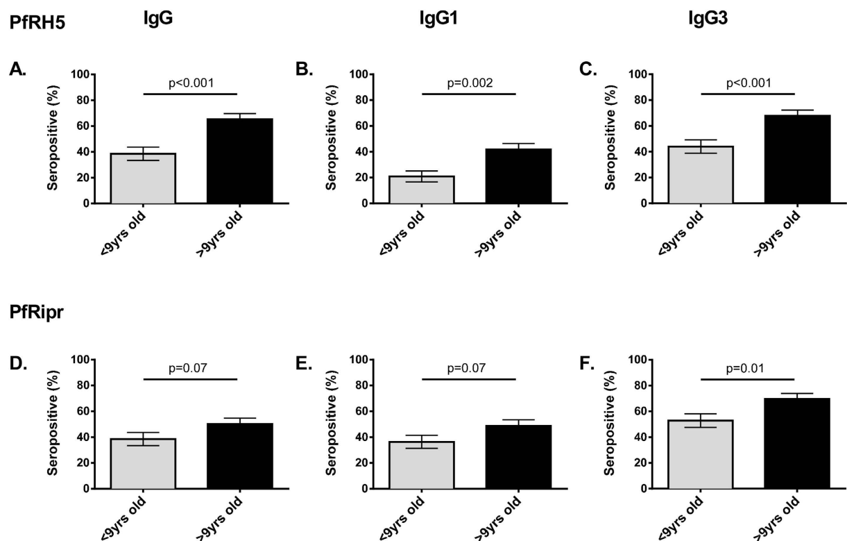
Figure 2. Seroprevalence of total IgG and subclass response to PfRH5 and PfRipr by age. IgG seroprevalence to PfRH5 and PfRipr recombinant proteins measured by ELISA. Results are shown as percentage seropositive.. Error bars indicate standard error of proportion (SE). Results are shown by Age ( \leq 9 or > 9 years of age). Top row: PfRH5. Bottom row: PfRipr. Results are shown for (A)/(D) Total IgG, (B)/(E). IgG1 and (C)/(F) IgG3 left to right. P values indicate chi square test.
