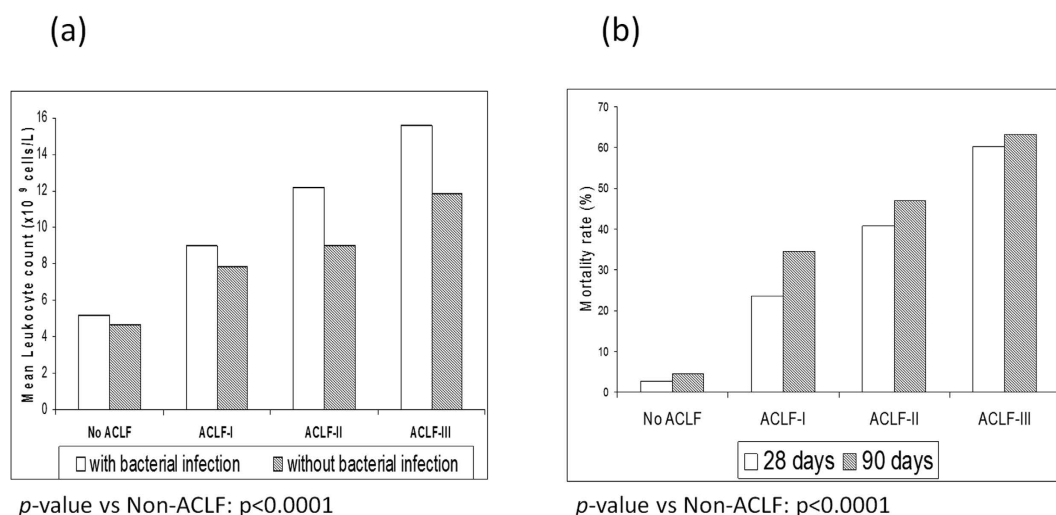
Figure 2. (A) Relationship between the severity of ACLF and the WCC.(B) Mortality rate at 28 days and 90 days according to the grade of ACLF.
