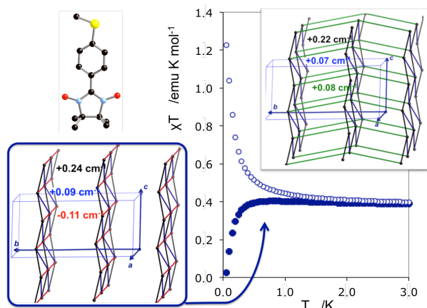
Figure 4. Calculated magnetic susceptibility \chi T(T) data for p-(methylthio)phenyl nitronyl nitroxide (see chemical formula inset, where hydrogen atoms are omitted for clarity) using the magnetic topology at 298 K (2D layer with competing FM and AFM interactions) and at 10 K (purely bulk FM).
