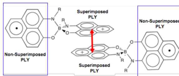
Figure 9. Scheme of the electronic structure of (a) the diamagnetic state (low temperature LT phase) and (b) the paramagnetic state (high temperature HT phase). The red arrow highlights the superposition of two cation PLY in the paramagnetic state
