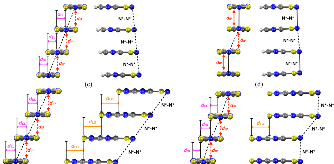
Figure 14. Two side views of a \pi -stack of the (a) HT and (b) LT polymorph of PDTA, and the (c) HT and (d) LT polymorph of TDPDTA. The d_{IP} , d_{SL} and d_{LG} variables measure the interplanar distance between adjacent radicals, the degree of latitudinal slippage between adjacent radicals, and the degree of longitudinal slippage, respectively. As may be seen in the images, the latitudinal slippage measures the degree of slippage with respect to the symmetry plane that is perpendicular to the molecular plane. The longitudinal slippage refers to the slippage along an orthogonal direction. Although not shown in the images, the structure of the \pi -stacks of TTTA and NCBDTA is very similar to that of PDTA. Figure adapted with permission of Ref. 114
