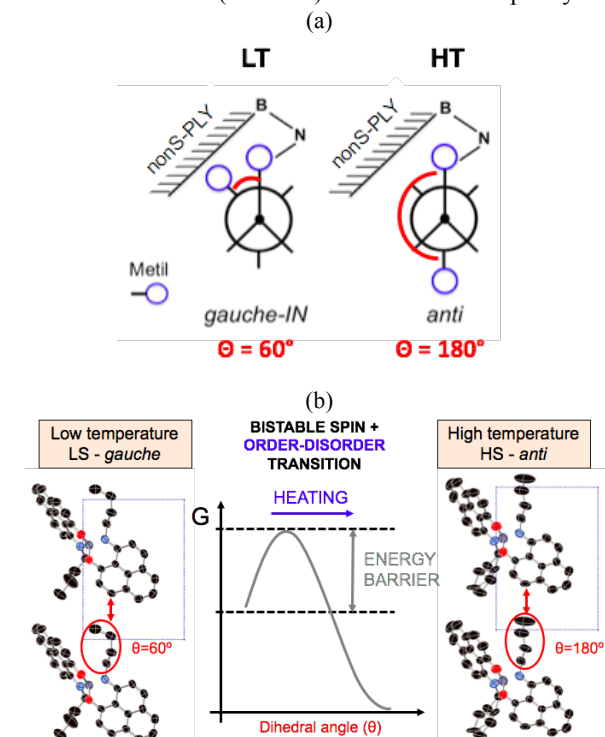
Figure 11. (a) Schematic illustration of the gauche- and anti-conformations of the LT (Low Temperature) and HT (High Temperature) phases of the butyl-substituted spiro biphenalenyl crystal. The acronym nonS-PLY stands for nonsuperimposed phenalenyl. (b) Scheme of the order-disorder phase transition originating the energy barrier and bistability in butyl-SBP.
