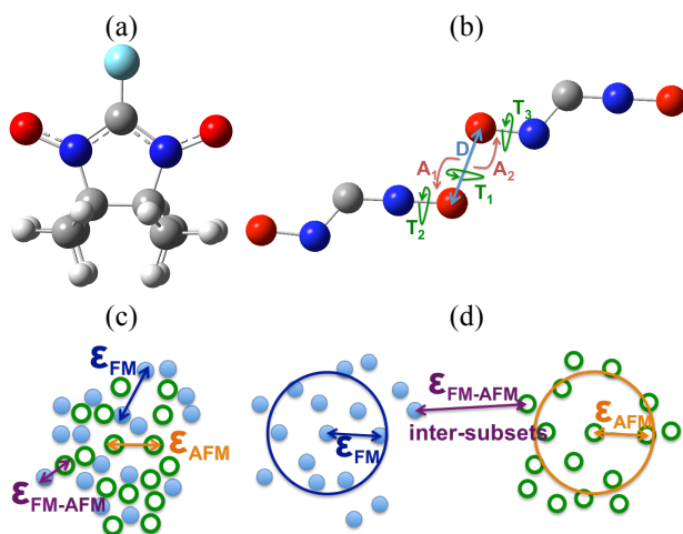
Figure 2. (a) General chemical formula of \alpha -nitronyl nitroxide radical. The unpaired electron is formally delocalised on the ONCNO fragment. (b) Coordinates used to define the inter-contact NO \cdots ON arrangement: D is the O \cdots O distance, A 1 and A 2 are the N-O \cdots O angles, T 1 is the N-O \cdots O-N dihedral angle, and T 2 , T 3 are the C-N-O \cdots O dihedral angles. Note that an equivalent set of coordinates was used to define C(sp 3 /sp 2 )-H \cdots O-N contacts. Cluster analysis resulting in (c) indistinguishable FM and AFM subsets (inter-subsets distances similar to intra-subset distances, \epsilon_{\text{FM-AFM}} \sim \epsilon_{\text{FM}}, \epsilon_{\text{AFM}} ), and (d) clearly separate FM and AFM subsets of crystals ( \epsilon_{\text{FM-AFM}} \gg \epsilon_{\text{FM}}, \epsilon_{\text{AFM}} )
