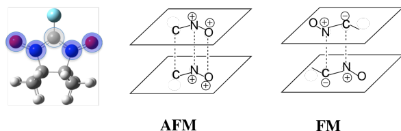
Figure 3. Spin density delocalised on the ONCNO group of an \alpha -nitronyl nitroxide radical. Positive spin density in blue and negative in grey. Schematic examples of AFM and FM coupling predicted by the McConnell-I model for dimers of \alpha -nitronyl nitroxide radicals.
