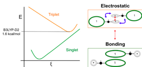
Figure 10. Left: Scheme of the potential energy landscape of the singlet and triplet states along the reaction coordinate that drives the spin transition. The adiabatic energy gap computed at B3LYP-D2 level is indicated. Right: Scheme of the electronic configuration and intermolecular interactions dominating the stability of the LS (bonding) and HS (electrostatic) states.
