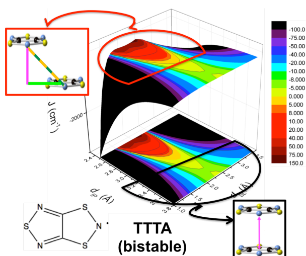
Figure 6. Magneto-structural correlation maps for TTTA (bistable). The FM and AFM fingerprint regions are shown in red and black, respectively
