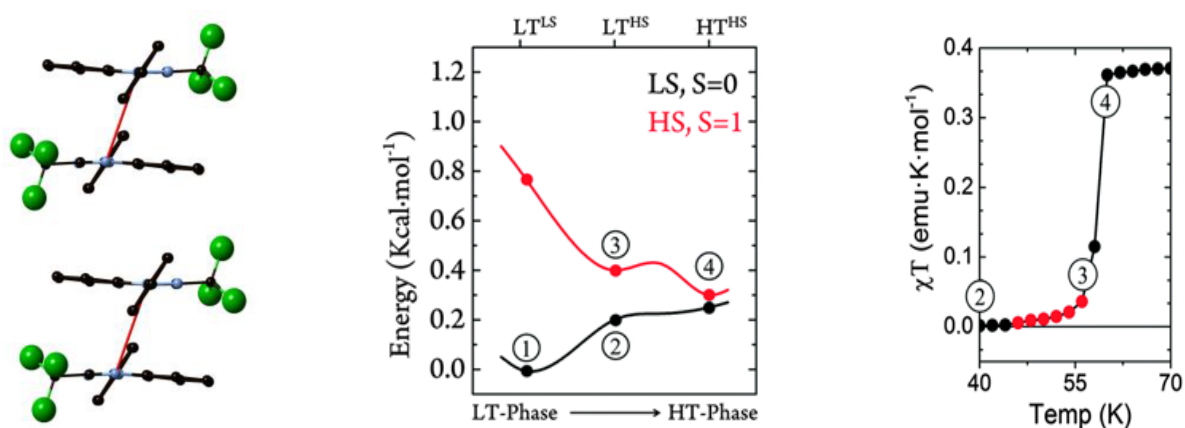
Figure 13. (left) HS- and LS-PES of dimers of B4 along the coordinate connecting the different minima. Energies are given per molecule. (right) Magnetic susceptibility curve of B4 around T_{1/2} . In red, we highlight the points with \chi T \neq 0 before the jump. The key steps of the phase transition are numbered in both plots, as discussed in the main text. Reprinted/adapted with permission from ref. 176 .
