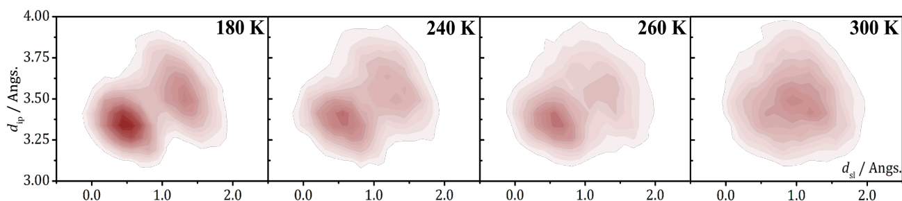
Figure 19. 2D-PDF's associated with the interplanar distance ( d_{ip} ) and the relative latitudinal slippage ( d_{sl} ) between adjacent NCBDTA radicals, as obtained from AIMD trajectories run at 180, 240, 260 and 300 K. Figure reprinted with permission of Ref. 112
