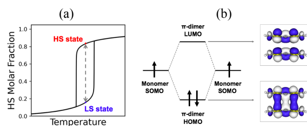
Figure 1. a) Schematic representation of the evolution of the high spin (HS) molar fraction upon increasing temperature. Inside the hysteresis region, both the low spin (LS) and HS states can be obtained ( i.e. bistability). b) Diagram of the frontier molecular orbitals of a pancake bond. The \pi -dimer of tetrathiafulvalene radical cation is shown where HOMO and LUMO orbitals are depicted.
