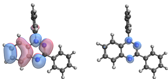
Figure 12. (left) SOMO orbital and (right) Spin Density in the Blatter radical
