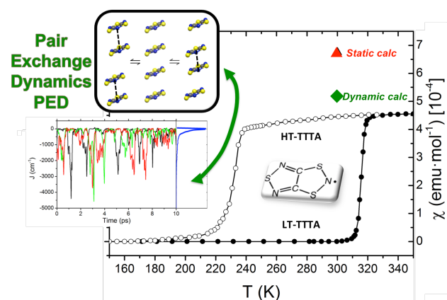
Figure 5. Magnetic susceptibility \chi(T) data for TTTA (see chemical formula inset, indicating the high-temperature HT and low-temperature LT polymorphs) using the magnetic topology at 300 K at static level (red symbol) and at dynamic level (green symbol). Note that the dynamic calculation (i.e. the vibrationally-averaged magnetic susceptibility data) is an improvement with respect to the static data. See inset regular \pi -stacks of the HT polymorph (top centre), which results from the dynamic interconversion between two distorted stacks (left- and right-hand side). Time-resolved fluctuations of J (in \text{cm}^{-1} ) and the corresponding probability distribution function (in blue) for the HT polymorph (where J (in red, green, black) stands for the magnetic coupling between any two adjacent radicals within a the \pi -stack shown in the figure).
