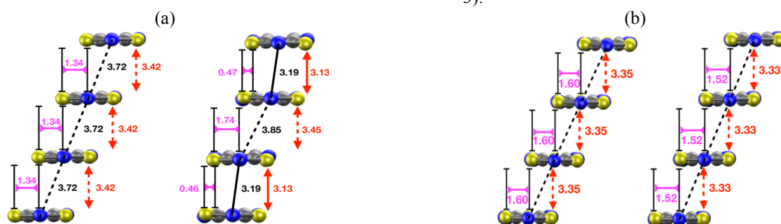
Figure 15. (a) Side view of a \pi -stack of the (left) X-ray-resolved structure at 323 K of the HT polymorph of PDTA and (right) the optimized structure at 0 K. Although not shown in the images, the structure of the \pi -stacks of TTTA and NCBDA is very similar to that of PDTA. (b) Side views of a \pi -stack of the (left) X-ray-resolved structure at 293 K of the HT polymorph of TDPDPA and (right) the optimized structure at 0 K. The black, red, purple and orange values shown in the image mark the distances between the nitrogen atoms of the S–N–S moieties of adjacent radicals, the interplanar distance between adjacent radicals and the degree of latitudinal and longitudinal slippage between adjacent radicals, respectively. Figures adapted with permission of Ref. 114
