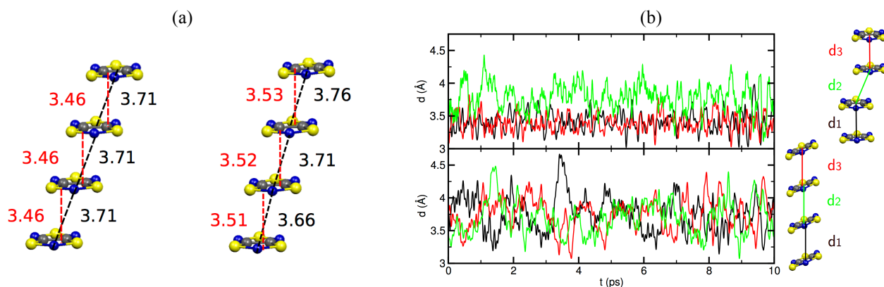
Figure 17. (a) Comparison between the structure of one stack of TTTA in the ( left ) X-ray resolved structure of the HT polymorph at 300 K and in the ( right ) average structure obtained from the AIMD simulations. The values marked in black and red refer to the N-N distance and the interplanar distance between adjacent radicals, respectively. (b) Time-resolved evolution of the distance between centroids of adjacent TTTA radicals in one of the stacks of the LT ( top ) and HT polymorph ( bottom ) of TTTA, as obtained from AIMD simulations run at 300 K. Figure adapted with permission of Ref. 109
