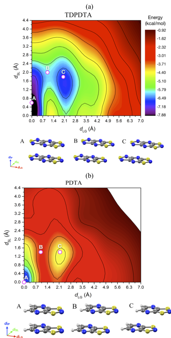
Figure 18. Potential energy surface of an (a) isolated \pi -dimer of TDPDTA radicals and (b) an isolated \pi -dimer of PDTA radicals as a function of the degree of latitudinal slippage ( d_{SL} ) and the degree of longitudinal slippage ( d_{LG} ), while keeping fixed the interplanar distance at values of 3.3 Å and 3.2 Å, respectively. The configurations associated with the A, B and C points marked on the color maps are displayed at the bottom of each color map. Figure adapted with permission of Ref. 114
