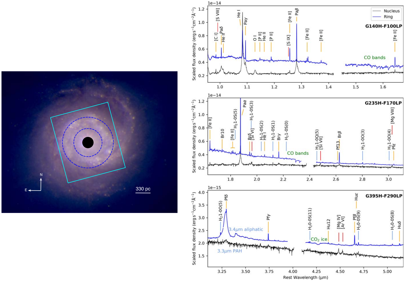
Figure 1. Left: HST (F110W) and JWST (F150W and F200W) color composite image of NGC 7469 (Bohn et al. 2023). North is up and east to the left, as indicated by the compass in the bottom left. Bright stellar clusters are detected throughout the starburst ring. The cyan rectangle indicates the combined field of view (FOV) of our dithered NIRSpec observations ( 4''.2 \times 4''.8 ). 1'' corresponds to 330 pc at the distance of the galaxy. The right panels show extracted NIRSpec spectra from the nucleus with a radius of 0''.4 (black) and the star-forming ring with inner and outer radius of 1'' and 1''.8 (blue). These extractions correspond to the black-filled circle and the dashed blue annulus in the galaxy image, respectively. The red, orange, and light blue lines indicate the location of the high ionization (coronal), the ionized, and molecular emission lines, respectively. The spectra were arbitrarily scaled for visualization purposes to differentiate between the nuclear and the star-forming ring spectra. The first shows the broad lines, typical of Type 1 nuclei, in the permitted emission lines as the hydrogen and helium recombination lines, high ionization coronal lines indicated by the red markers, and other emission lines such as [Fe II] and H_2 . The latter is dominated by narrow lines, a prominent PAH feature at 3.3 \mu\text{m} close to an aliphatic feature at 3.4 \mu\text{m} , CO stellar absorption features, and \text{CO}_2 absorption.
