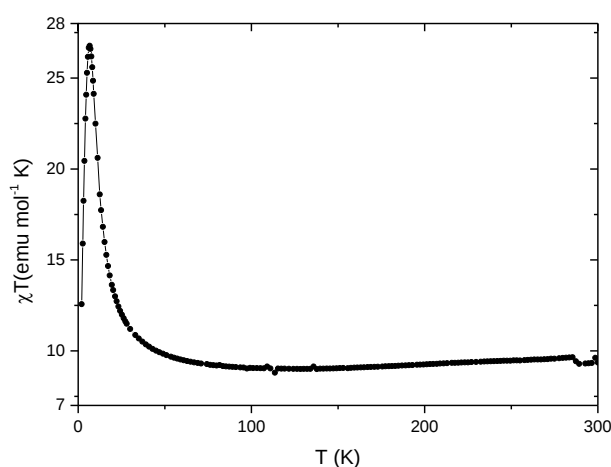
Figure 3. Temperature dependence of the product of the molar magnetic susceptibility times the temperature ( \chi_{\text{m}}T ) of 1 under an applied field of 1000 Oe.
