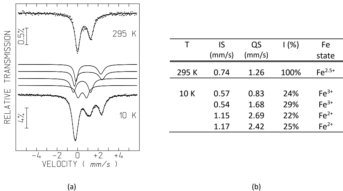
Figure 6. (a) Mössbauer spectra of 1 taken at 295 and 10 K and (b) estimated parameters from the spectra. The lines over the experimental points are the calculated functions. On the spectrum taken at 10 K this function is the sum of four quadrupole doublets shown slightly shifted for clarity. IS, isomer shift relative to metallic \alpha -Fe at 295 K; QS, quadrupole splitting; I, relative areas. Estimated errors are < 0.02 mm/s for IS, QS, < 2\% for I.
