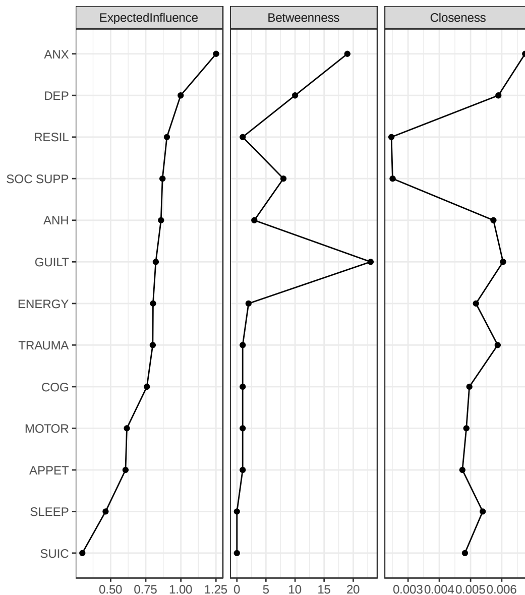
Figure 2. Centrality Plots for EBICglasso network depicting the expected influence, betweenness and closeness of each node (variable). Abbreviations: GAD-7 total score, ANX: anxiety; PHQ-8 items, DEP: "sad mood"; ANH: "anhedonia"; ENERGY: "energy"; TRAUMA: Trauma; COG: "concentration"; GUIL: "guilty"; MOTOR: "motor"; APPET: "appetite"; SLEEP: "sleep"; CD-RISC total score, RESIL: "resilience"; OSSS-3 total score, SOC SUPP: "Social Support"; C-SSRS score, SUIC: suicidal behavior.
