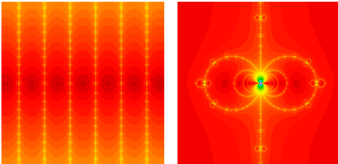
FIGURE 4. Left: The dynamical plane of the map f from Example 7.2, showing the invariant attracting basins U_k . Right: Zoom of the dynamical plane near a pole p_k .
