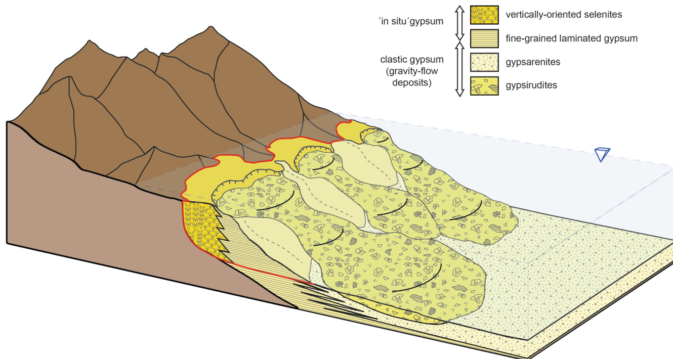
Fig. 10. Depositional model for MSC gypsum deposits of the Kalavassos Fm. in the North Cyprus Mesaoria basin.
