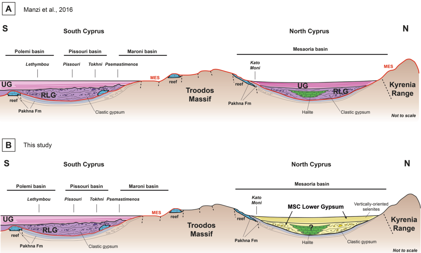
Fig. 13. Schematic geological section of MSC gypsum deposits (Kalavassos Fm.) in South and North Cyprus. A: Manzi et al. (2016); B: This work.
