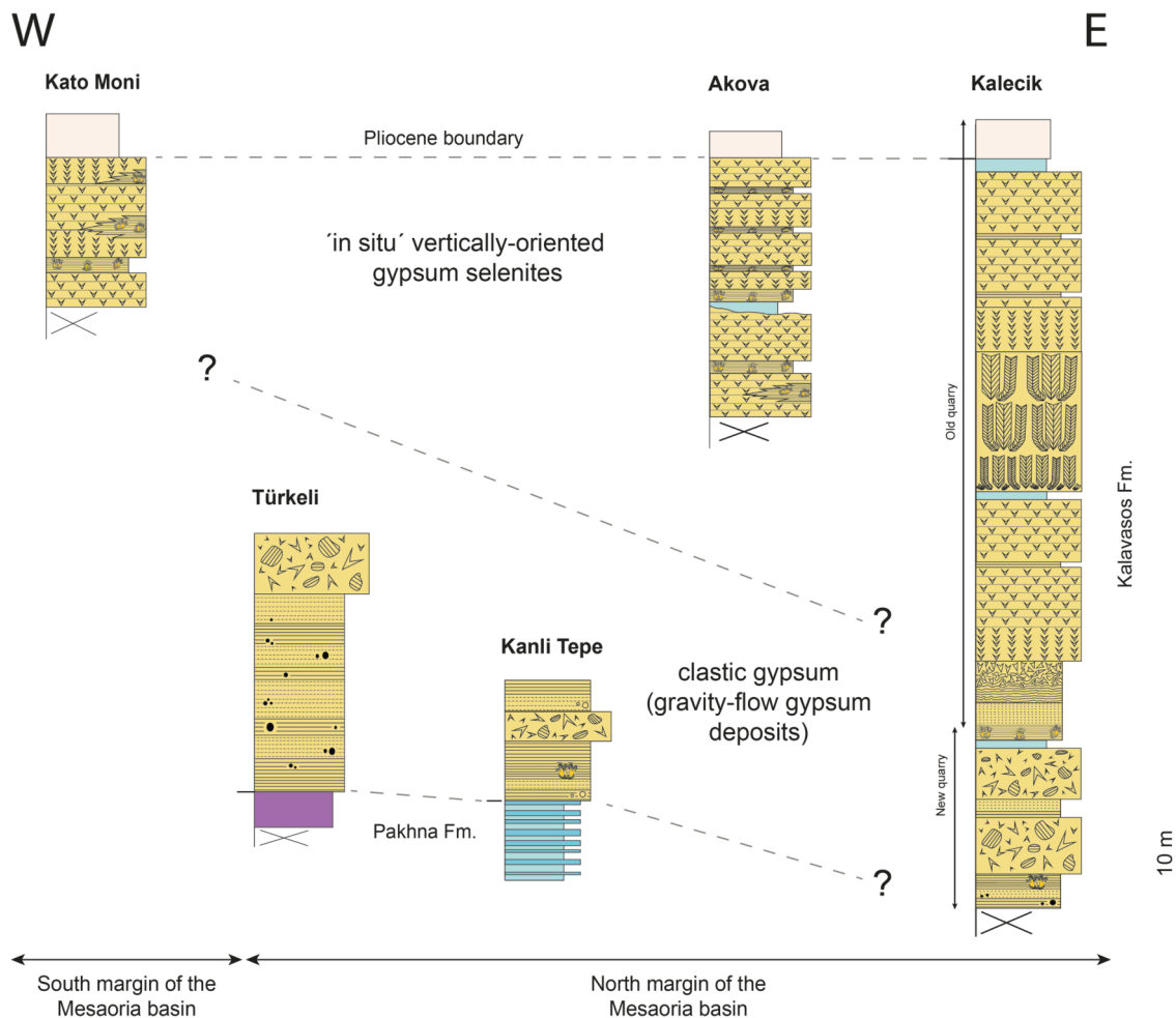
Fig. 11. Correlation chart of MSC gypsum sections of the Kalavassos Fm. in the Mesaoria basin (North Cyprus).
