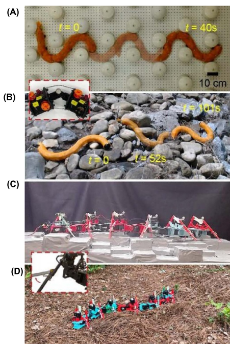
Figure 30. Examples of mechanically intelligent devices. (A), (B) A robophysical model of a bilaterally actuated undulating robot leverages the redundancy of its multi-joint architecture and the asymmetric compliance to confront (A) lab and (B) natural terrain through mechanical intelligence. From [191]. Reprinted with permission from AAAS. The inset shows a close-up on the multi-joint architecture. (C), (D) A centipede robot similarly leverages both the redundancy of its legs and the asymmetric compliance its limb joints in (C) lab (From [192]. Reprinted with permission from AAAS) and (D) natural settings. The inset shows a close-up on the limb joints. © (2020) IEEE. Reprinted, with permission, from [193].
