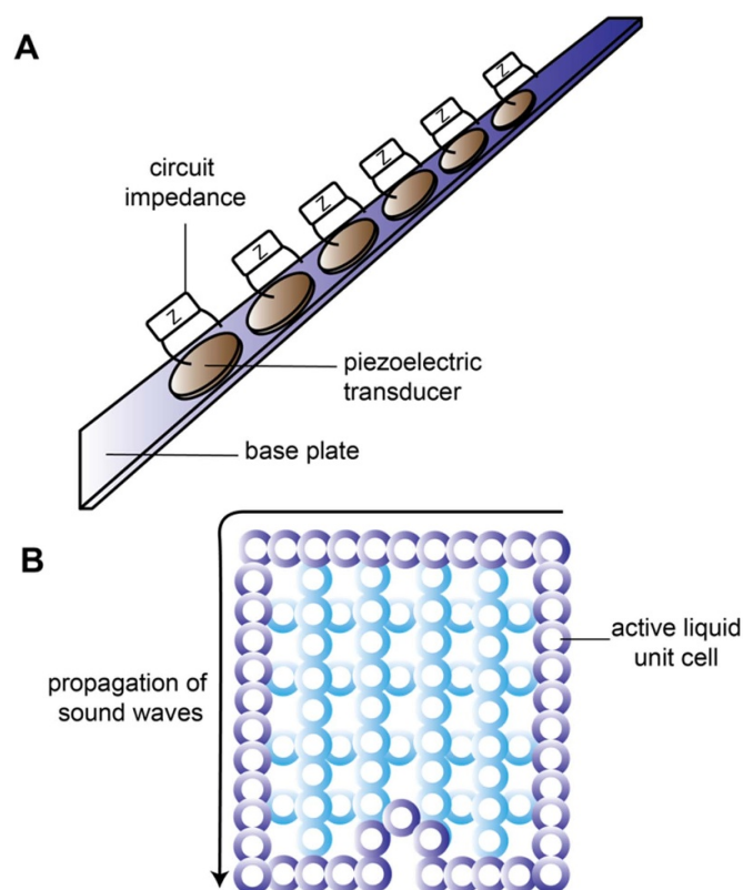
Figure 25. Schematics of two active acoustic metamaterials. (A) Active acoustic metamaterial using external electric field through piezoelectric unit cells [156]. The piezoelectric local resonators can tune the stiffness of the host structure and tailor the acoustic wave propagation behaviour. (B) An animate acoustic metamaterial consisting of active liquid unit cells, enabling topological acoustic property [157]. The liquid unit cells control the propagation of sound and enable topological insulators which are immune to structural defects. The high-density active particles in the unit cells are shown in dark blue and low-density active particles are shown in light blue.
