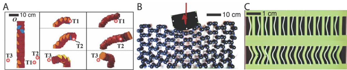
Figure 27. Examples of active mechanical metamaterials. (A) Example of a shape-changing metamaterial made from an origami unit cell. The metamaterial consists of a pneumatically actuated origami, which is only actuated via a single pressure source. It can bend and twist such that the top of the column can reach points T1, T2 and T3 only by adjusting the history of the pressure loading. Left panel: metamaterial at rest; middle panel: simulations; right panel: experiments [182]. John Wiley & Sons. © 2022 Wiley-VCH GmbH. (B) Example of an active metamaterial deflecting a projectile. The metamaterial consists of 120 robotic hexagons made from building blocks that break reciprocity. The metamaterial as a whole is described by a generalization of elasticity called odd elasticity. Odd elasticity leads to non-reciprocal coupling between the two shear modes of the material when perturbed by the projectile and, in turn, to deflect the projectile [175]. (C) Example of a multistable metamaterial performing a counting task under cyclic compression. The metamaterial consists of a series of thin and thick beams. The thick beams are designed to be asymmetric: they buckle initially towards the left, but once nudged by the thin beams, they snap towards the right, in turn making the adjacent thin beam on their right snap. The metamaterial at the smallest (top panel) and largest (bottom panel) compression of cycle 2 [180].
