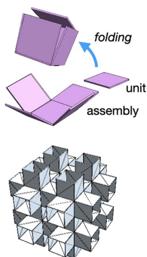
Figure 18. Self-assembling tiles to generate complex or actuating structures. (Top) Self-assembly is an alternate pathway to forming complex origakata at the nanoscale. This can produce origami-like structures that cannot be folded from a flat sheet without gluing. (Bottom) A model of a triply-periodic orikata that can be formed with triangular units having the symmetry cubic symmetry. This cannot be folded from a flat sheet of paper but could be assembled from triangular units following simple rules.
