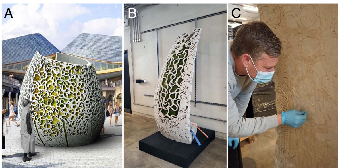
Figure 35. Probiotic building prototypes. (A) Rendering of an imagined probiotic pavilion structure. (B) 1:1 scale 3D printed, microbially active building prototype, embedded with bryophytes (outer facing) and soil microbes (inner facing). (C) Photograph of prototype undergoing a microbiome monitoring study using 16 S DNA sequencing.
