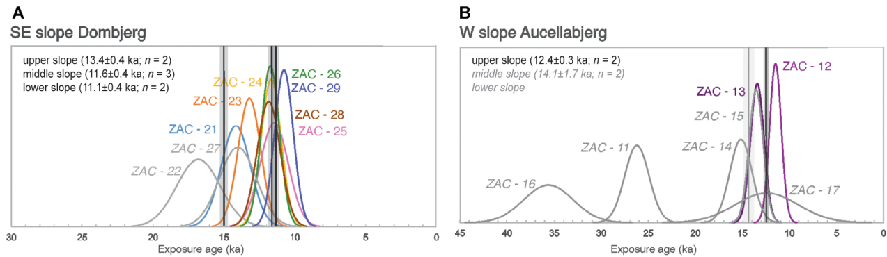
Fig. 6. A. Probability distribution functions of ^{10}\text{Be} ages from SE Domjerg slope (Zackenberg Valley) that have metamorphic bedrock. B. Probability distribution functions of ^{10}\text{Be} ages from west Aucellabjerg slope (Zackenberg Valley) that have sedimentary bedrock (modified from Garcia-Oteyza et al. (2022), see this original publication for the exact location of the samples).
