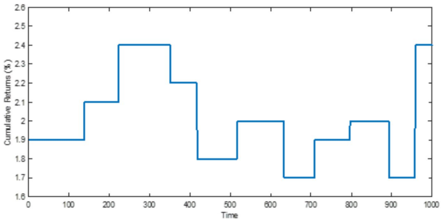
Fig. 17 Cumulative Returns (threshold=0.00025) using ARMA-GARCH-NN
