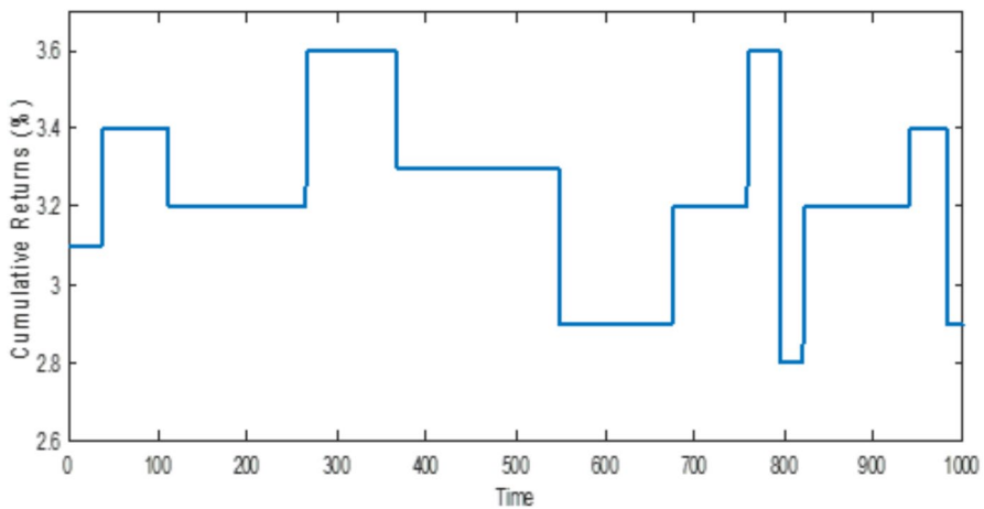
Fig. 16 Cumulative Return under Different Thresholds using ARMA-GARCH-F-QRNN
