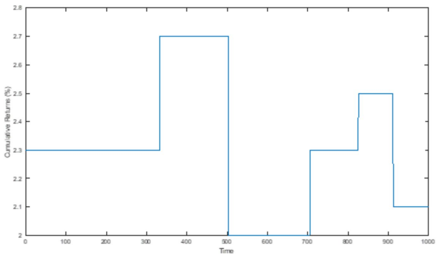
Fig. 27 Cumulative Return under Different Thresholds using MS-ARMA-GARCH-RBF
