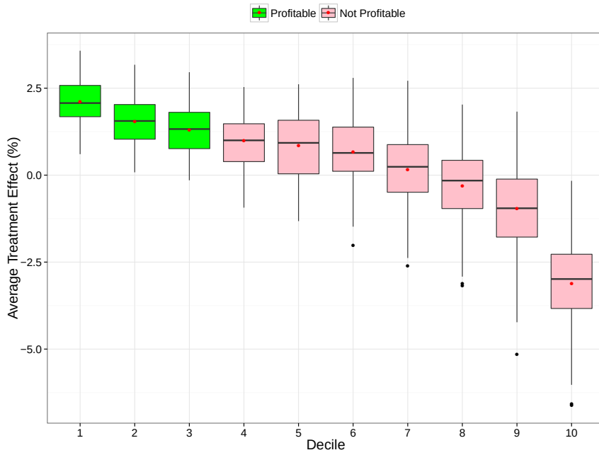
Figure 3: Boxplots of the actual average treatment effect for each decile based on 100 random training/validation data splits. The first (tenth) decile represents the 10% of clients with highest (lowest) predicted personalized treatment effect. Clients with higher estimated personalized treatment effect were, on average, positively influenced to buy as a result of the marketing intervention activity.
