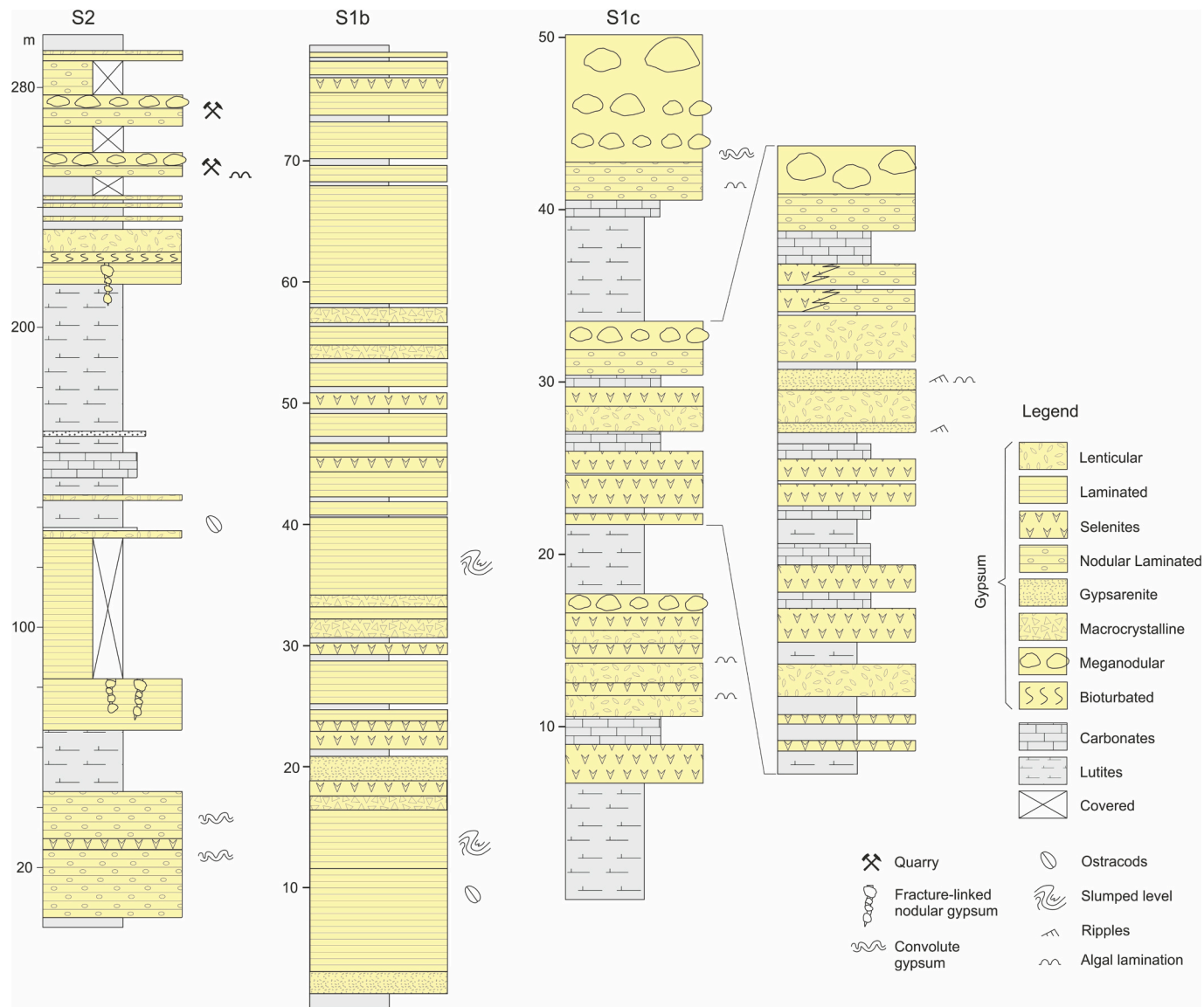
Fig. 9. Stratigraphic sections showing the distribution of the gypsum lithofacies.
