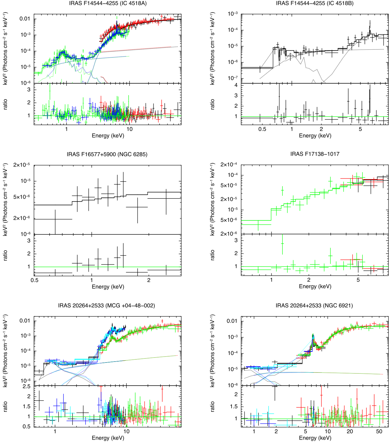
Figure B3. X-ray spectra of IC 4518A [ NuSTAR and XMM-Newton ; Section A21, N_H = (2.4 \pm 0.2) \times 10^{23} \text{ cm}^{-2} ], IC 4518B [ XMM-Newton ; Section A21, N_H = (3.2^{+4.1}_{-1.4}) \times 10^{23} \text{ cm}^{-2} ], NGC 6285 ( Chandra , Section A24), IRAS F17138-1017 ( NuSTAR and Chandra ; Section A25), MCG +04-48-002 [ NuSTAR and XMM-Newton , Section A26, N_H = (5.8^{+0.7}_{-0.4}) \times 10^{23} \text{ cm}^{-2} ], and NGC 6921 ( NuSTAR and XMM-Newton , Section A26, N_H = (1.78^{+0.30}_{-0.53}) \times 10^{24} \text{ cm}^{-2} ).
