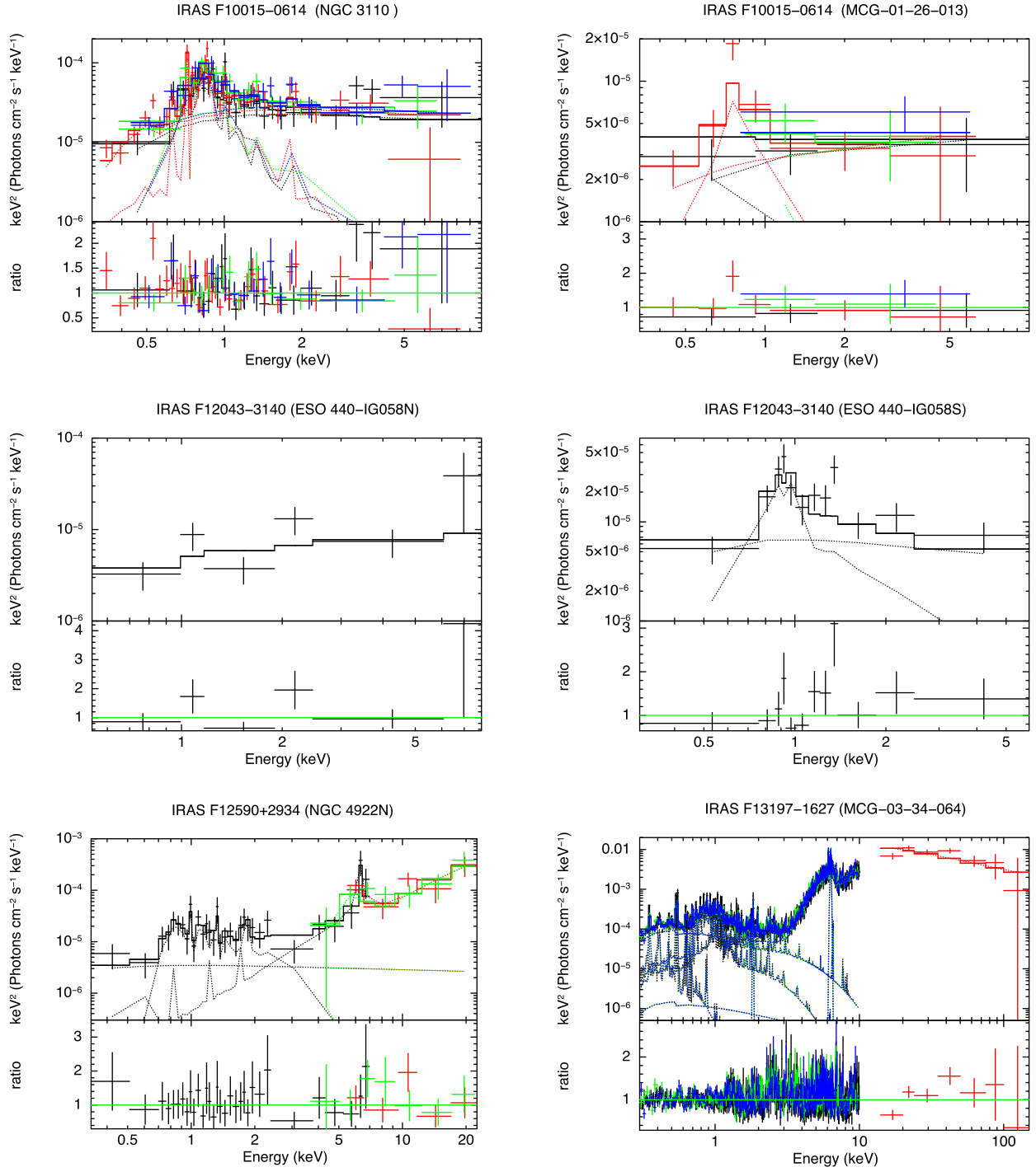
Figure B2. X-ray spectra of NGC 3110 ( XMM-Newton and Chandra ; Section A10), MCG-01 – 26 – 013 ( XMM-Newton and Chandra , Section A10), ESO 440-IG058N ( Chandra ; Section A14), ESO 440-IG058S ( Chandra ; Section A14), NGC 4922N ( NuSTAR and Chandra ; Section A16, N_{\text{H}} \geq 4.27 \times 10^{24} \text{ cm}^{-2} ), and MCG-03 – 34 – 064 [ XMM-Newton EPIC and Swift /BAT; Section A18, N_{\text{H}} = (54.2^{+0.7}_{-0.9}) \times 10^{22} \text{ cm}^{-2} ].
