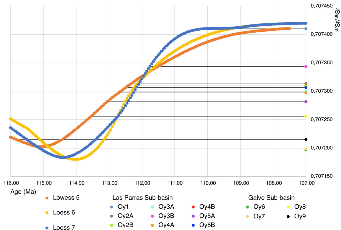
FIGURE 8. ^{87}\text{Sr}/^{86}\text{Sr} variations in seawater around the Aptian–Albian boundary for the LOWESS/LOESS look-up tables 5, 6, and 7 of McArthur et al. (2012), McArthur et al. (2020) and McArthur and Howarth (2024), respectively. The corrected ^{87}\text{Sr}/^{86}\text{Sr} ratios obtained from the samples are plotted, and the intersection between the sample ratios and the curves indicates the corresponding numerical ages, shown on the horizontal axis. The numerical age of the Aptian–Albian boundary is 113Ma and 113.2Ma according to the Geological Time Scale 2012 (Gradstein et al., 2012) and the Geological Time Scale 2020 (Gradstein et al., 2020), respectively.
