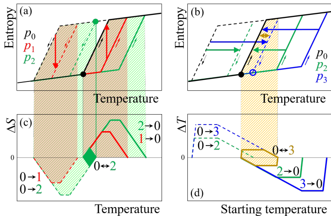
Fig. 1 Schematic representations of isobaric entropy-temperature curves and conventional BC effects to evaluate reversibility. (a,b) Isobaric entropies at different values of pressure p_0 (black), p_1 > p_0 (red), p_2 > p_1 (green) and p_3 > p_2 (blue) on heating (continuous lines) and on cooling (dashed lines) as indicated by the small arrows. In both panels, black filled circles denote the onset of the endothermic transition at pressure p_0 [ T_{I \rightarrow I}(p_0) ]. In panel (a) the green filled circle denotes the onset of the exothermic transition at p_2 , T_{I \rightarrow II}(p_2) . In panel (b) the blue empty circle denotes the finishing temperature of the transition on cooling at pressure p_3 , T_{II \rightarrow I}^f(p_3) . In panel (a), the red vertical downward (upward) arrow indicates the thermodynamic path used to calculate irreversible isothermal entropy changes \Delta S on compression (decompression). In panel (b), the horizontal rightward (leftward) arrows indicate the thermodynamic paths used to calculate irreversible adiabatic temperature changes \Delta T on compression (decompression). The left-right yellow arrow indicates the thermodynamic path used to calculate reversible \Delta T . (c) Irreversible \Delta S obtained under a pressure increase of p_1 - p_0 (red, dashed), under an increase of p_2 - p_0 (green, dashed), under a decrease of p_0 - p_1 (red, continuous) and under a decrease of p_0 - p_2 (green, continuous). The green colored area indicates the reversible \Delta S obtained from overlapping the curves obtained on increasing and decreasing the field. (d) Irreversible \Delta T obtained under a pressure increase of p_2 - p_0 (green, dashed), under an increase of p_3 - p_0 (blue, dashed), under a decrease of p_0 - p_2 (green, continuous) and under a decrease of p_0 - p_3 (blue, continuous). The dark yellow line indicates the reversible \Delta T . Notice that \Delta T are plotted as a function of the starting temperature because the system temperature changes along the adiabatic path.
