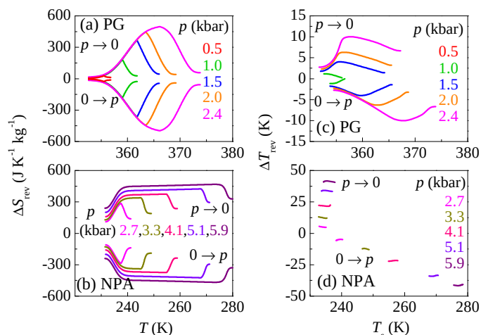
Fig. 5 (a,b) Reversible isothermal entropy changes as a function of temperature and (c,d) reversible adiabatic temperature changes as a function of the starting temperature T_s , under application and removal selected pressures in (a,c) PG and (b,d) NPA. For NPA, \Delta T_{\text{rev}} is shown only within the temperature interval where the adiabatic path starts and finishes at the transition.
