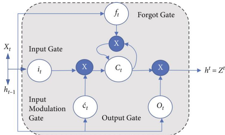
Figure 3. LSTM Cell Unit Representation. Source: (Tomar et al. 2022).
