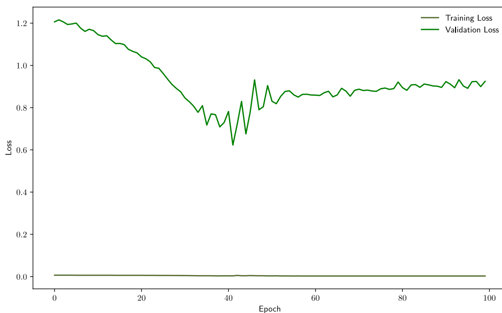
Figure 11. Training and Validation Loss Over Epochs. Source: Own Preparation.
