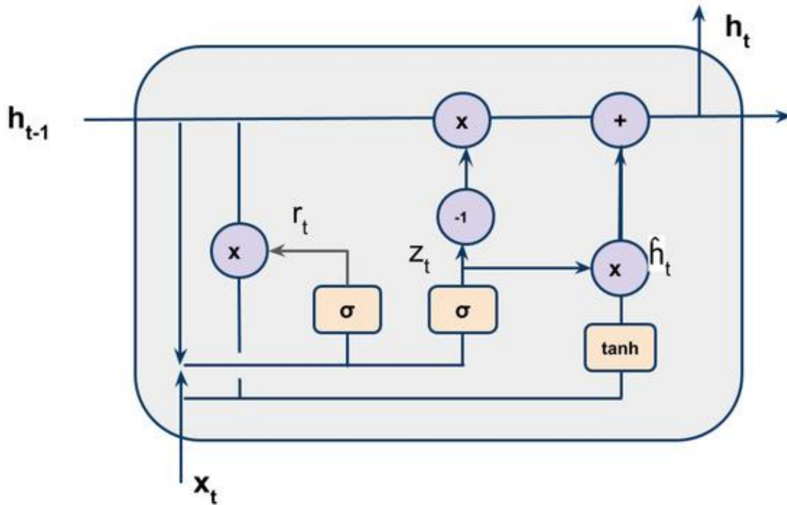
Figure 2. GRU Cell Unit Representation. Source: (Hosseini et al. 2020).
