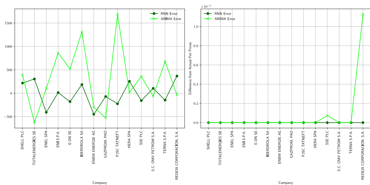
Figure 14. Differences in Call and Put Option Prices. Source: Own Preparation.
