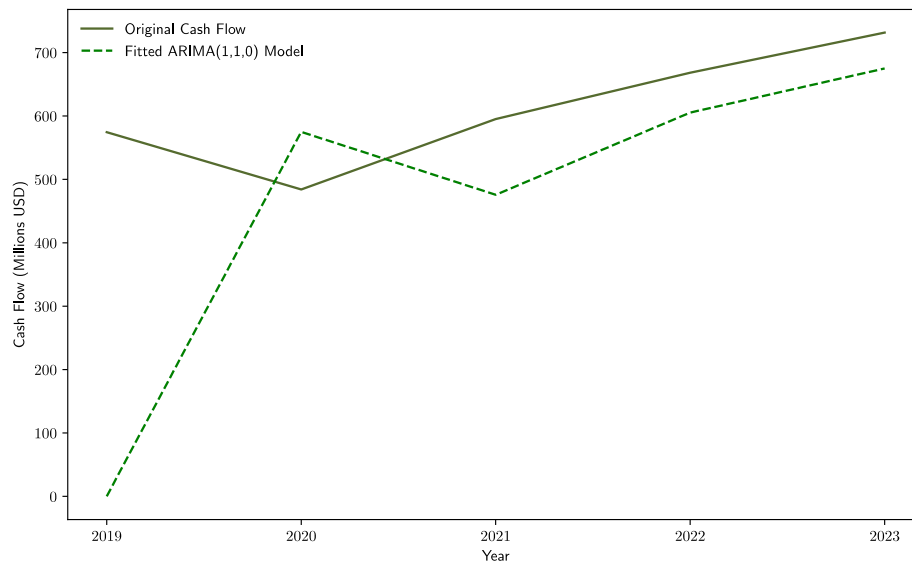
Figure 7. ARIMA(1,1,0) Model Fit for Romgaz S.A. Source: Own Preparation.
