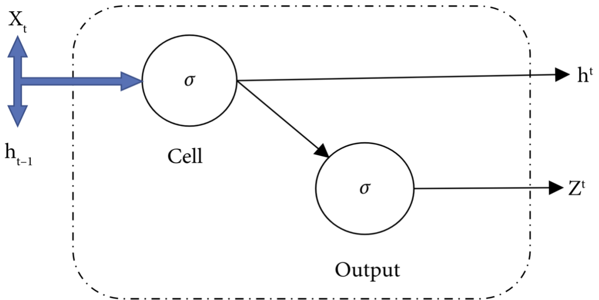
Figure 1. RNN Cell Unit Representation Source: (Tomar et al. 2022).
