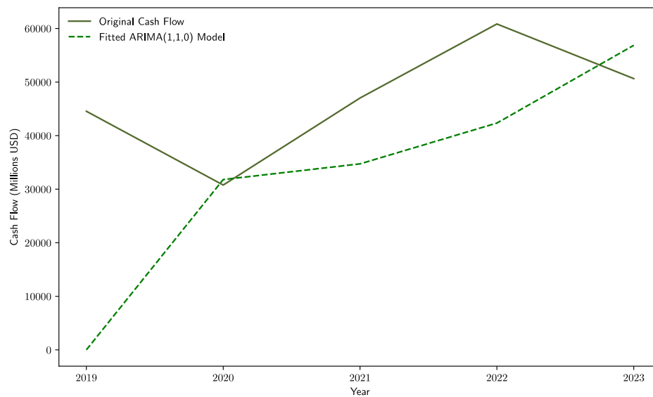
Figure 8. ARIMA(1,1,0) Model Fit for Shell plc. Source: Own Preparation.
