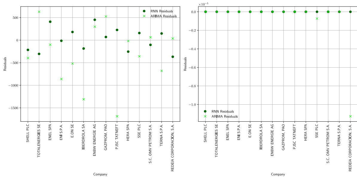
Figure 13. Residuals of Call and Put Option Prices. Source: Own Preparation.
