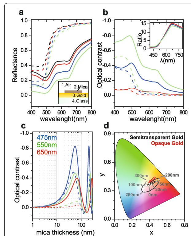
Figure 1 Calculated reflectance spectra, optical contrasts, and color evolution of the mica flakes. (a) Calculated reflectance spectra of mica (colored lines) and gold (black lines) in the structure shown in the inset as a function of the wavelength of visible light. Mica thicknesses are 0 nm (black lines, bare gold), 10 nm (red lines), 30 nm (blue lines), and 50 nm (green lines). Gold layer thicknesses are 20 nm (continuous lines) and 300 nm (dashed lines). Inset: schematic representation of the layered structure analyzed. (b) Optical contrast in reflection mode between the mica and gold parts of the sample as a function of the wavelength of light for the same cases considered in (a). Inset: ratio between the contrasts for the two gold layer thicknesses considered. (c) Optical contrast in reflection mode as a function of mica thickness for three representative wave lengths, 475 nm (blue lines), 550 nm (green lines), and 650 nm (red lines), and two gold layer thickness, 20 nm (continuous lines) and 300 nm (dashed lines). (d) Evolution of the mica color (lines) as a function of its thickness in the xy chromatographic space for the case of semitransparent (black line) and opaque (red line) gold substrates.
