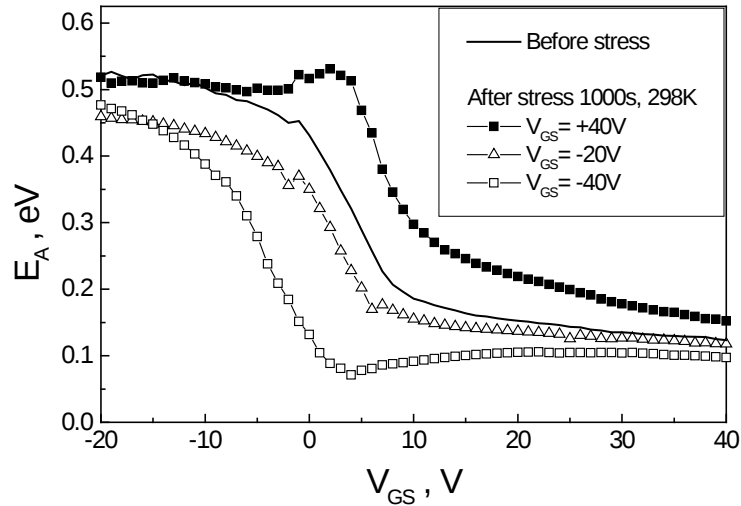
Fig.2. Dependence of the activation energy ( E_{\text{ACT}} = E_{\text{C}} - E_{\text{F}} ) of the sub-threshold transfer characteristics for TFT stressed at different gate biases.
