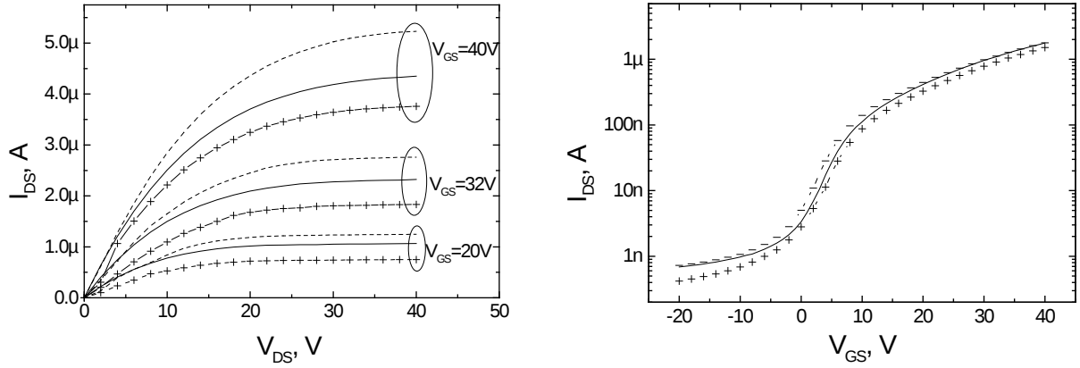
Fig. 1. Output and transfer characteristics of nano-crystalline TFT measured as-deposited (solid lines) and after different gate bias stress: V_{\text{GS}} = +40 V (- symbols), V_{\text{GS}} = -40 V (+ symbols).
