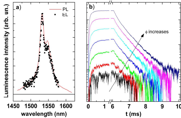
Fig. 2. a) Electroluminescence spectra of layer C352 (squares). A photoluminescence spectrum has been superimposed (red line) for comparison. b) Electroluminescence versus time for increasing flux (as symbolised by the arrow) from 7 \times 10^{13} \text{ cm}^{-2}.\text{s}^{-1} to 4 \times 10^{16} \text{ cm}^{-2}.\text{s}^{-1} .
