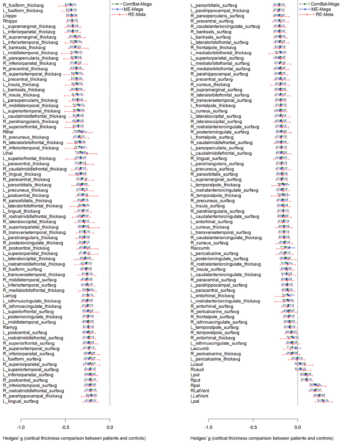
Fig. 2. Forest plot for random-effect meta-analysis (light red), mixed-effects mega-analysis (blue) and ComBat mega-analysis (dark green).
