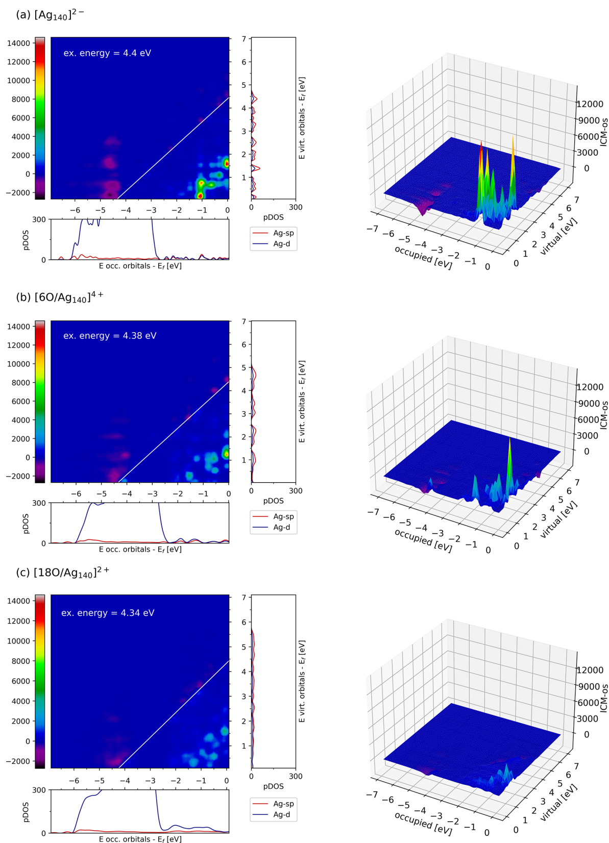
Figure 7. ICM-OS of \text{Ag}_{140} , 6\text{O}/\text{Ag}_{140} , and 18\text{O}/\text{Ag}_{140} for excitation energies of 4.4, 4.38, and 4.34 eV, respectively. Orbital energies are shifted with respect to HOMO (i.e., the Fermi level). For each system, the DOSs projected on the sp or d states of Ag are plotted along the axes of the ICM-OS. 3D versions of the plots are also included (right-hand panels) for clarity.
