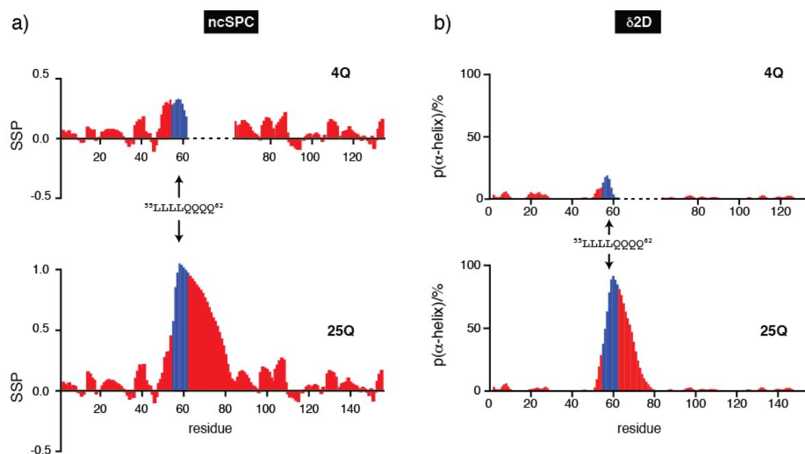
Figure 3. Secondary structure propensity of 4Q and 25Q obtained by using ncSPC (a) and population of \alpha -helix obtained by using \delta 2D (b). To facilitate the comparison, values for residues of 4Q which follow the polyQ tract are shifted to the right by 21 units. Values for residues 55 to 62, corresponding to the ^{55}\text{LLLL}^{58} motif and the first 4 Gln of the polyQ tract, are shown in blue to highlight the variation of the structural properties of the protein due to the different length of the polyQ tract.
