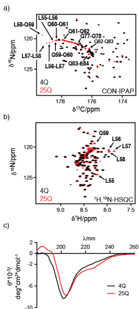
Figure 2. Comparison of the NMR (a,b) and CD (c) spectra of 4Q and 25Q. Central region of (a) the CON-IPAP spectrum and (b) the ^1\text{H} - ^{15}\text{N} HSQC spectrum of 400 \mu\text{M} 4Q (black) and 25Q (red) at 278 K with an indication, in panel b, of the resonances which experience the largest chemical shift variations upon increasing the length of the polyQ tract. A close up of the CON-IPAP spectrum of 25Q with the full assignment of the polyQ tract is provided as supplemental material (Fig. S2). c) CD spectrum of 120 \mu\text{M} 4Q and 130 \mu\text{M} 25Q at 310 K.
