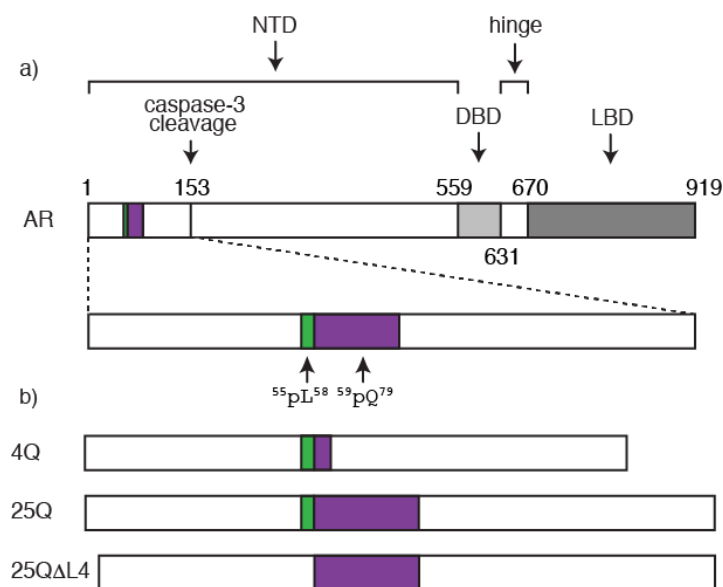
Figure 1. Structural organization of AR. a) Position of the transactivation (NTD), DNA binding (DBD) and ligand binding (LBD) domains of AR with an indication of the positions of the 55 LLLL 58 motif, shown in green, of the polymorphic polyQ tract, shown in purple, and of the caspase 3 cleavage site. b) AR constructs used in this work (see also Fig. S1).
