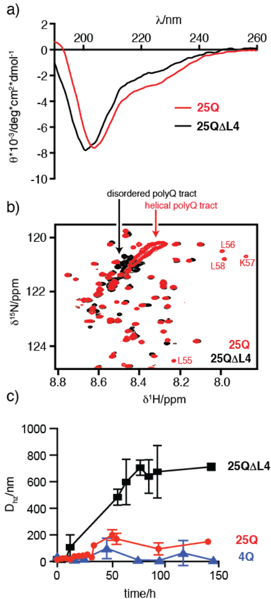
Figure 4. Characterization of the structural and aggregation properties of 25Q (red) and 25Q \Delta L4 (black). a) Comparison of the CD spectra of 130 \mu M 25Q and 140 \mu M 25Q \Delta L4 at 310K. b) Comparison of the ^1\text{H} - ^{15}\text{N} HSQC NMR spectra of 50 \mu M 25Q and 43 \mu M 25Q \Delta L4 at 278K. The cross-peaks belonging to the four Leu of 25Q immediately preceding the polyQ tract, not present in 25Q \Delta L4, are indicated. The absence of helical propensity in 25Q \Delta L4, which reduces the chemical shift dispersion of the resonances corresponding to the polyQ tract, is highlighted. c) Temporal evolution of the mean particle size of 4Q (blue), 25Q and 25Q \Delta L4 at 20 \mu M and 310K.
