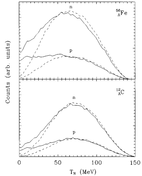
FIG. 7. Effect of the final state interactions in the spectrum of nucleons emitted in the 1N -induced decay of ^{56}_{\Lambda}\text{Fe} and ^{12}_{\Lambda}\text{C} . Dashed line: results without FSI's. Solid line: results including FSI's. The results have been obtained for a value \Gamma_n/\Gamma_p=1 .
