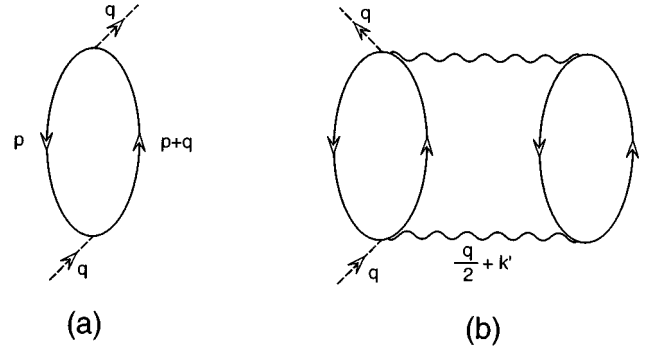
FIG. 3. Diagrams employed in the evaluation of \text{Im}\bar{\Pi}_{1p1h}^* (a) and \text{Im}\bar{\Pi}_{2p2h}^* (b).
