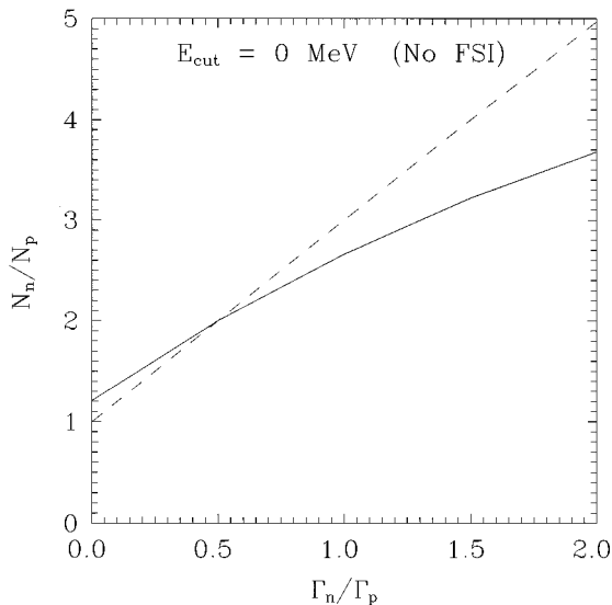
FIG. 9. N_n/N_p as a function of \Gamma_n/\Gamma_p in the decay of ^{12}\text{C} with no cut in the detection energy and no final state interactions. Dashed line: 1N -induced mechanism. Solid line: (1N+2N) -induced mechanisms.
