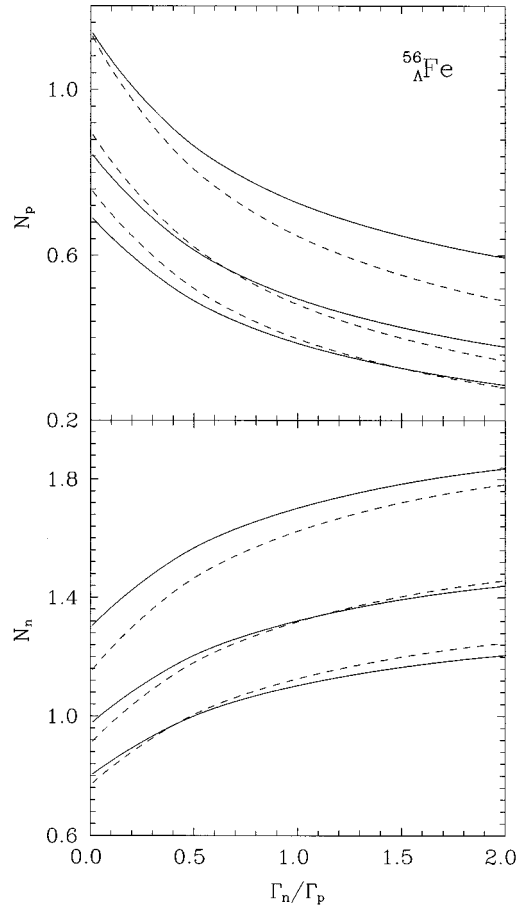
FIG. 14. Same as Fig. 12 but for ^{56}_{\Lambda}\text{Fe} .
