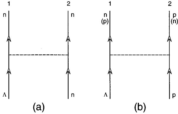
FIG. 4. Feynman diagrams for the transition \Lambda N \rightarrow NN : neutron-induced \Lambda decay (a) and proton-induced \Lambda decay (b).
