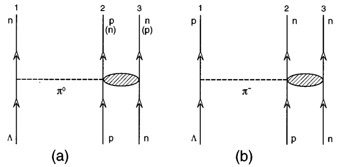
FIG. 5. Feynman diagrams for the two-nucleon-induced \Lambda decay through virtual \pi^0 absorption (a) and virtual \pi^- absorption (b).
