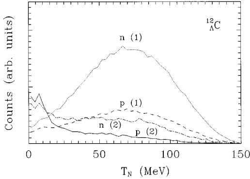
FIG. 6. Spectra of neutrons and protons in the decay of ^{12}_{\Lambda}\text{C} . Dashed line: protons from the 1N -induced mechanism. Dotted line: neutrons from the 1N -induced mechanism. Solid line: protons from the 2N -induced mechanism. Dash-dotted line: neutrons from the 2N -induced mechanism. The results have been obtained for a value \Gamma_n/\Gamma_p=1 .
