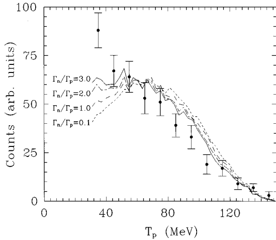
FIG. 15. Proton spectrum for different values of \Gamma_n/\Gamma_p in the decay of ^{12}_{\Lambda}\text{C} . The experimental points are taken from Ref. [4].
