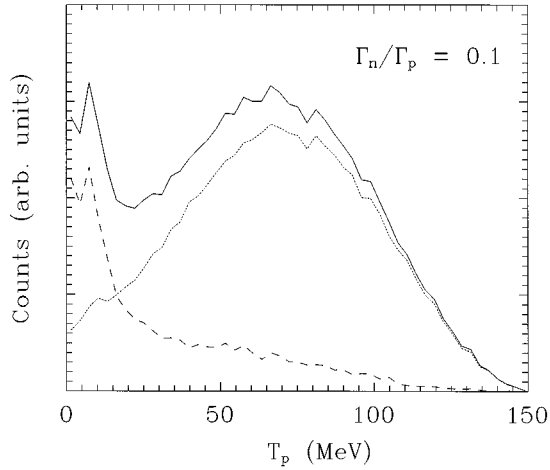
FIG. 8. Proton spectrum in the decay of ^{12}\text{C} , obtained for a value \Gamma_n/\Gamma_p=0.1 . Dotted line: 1N -induced mechanism. Dashed line: 2N -induced mechanism. Solid line: total.
