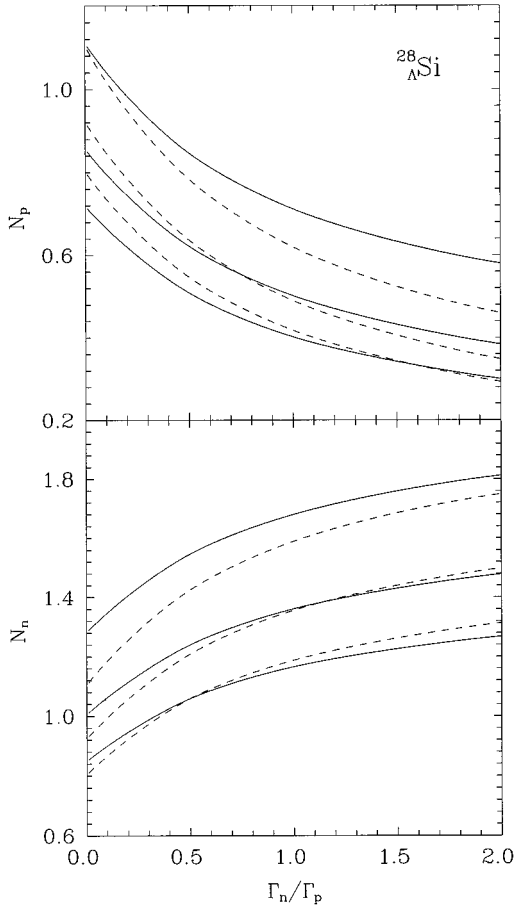
FIG. 13. Same as Fig. 12 but for ^{28}_{\Lambda}\text{Si} .
