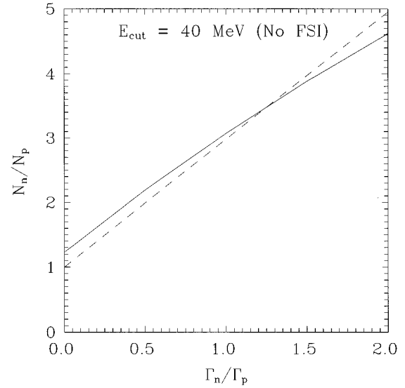
FIG. 10. Same as Fig. 9, but with a detection threshold of 40 MeV and no final state interactions.
