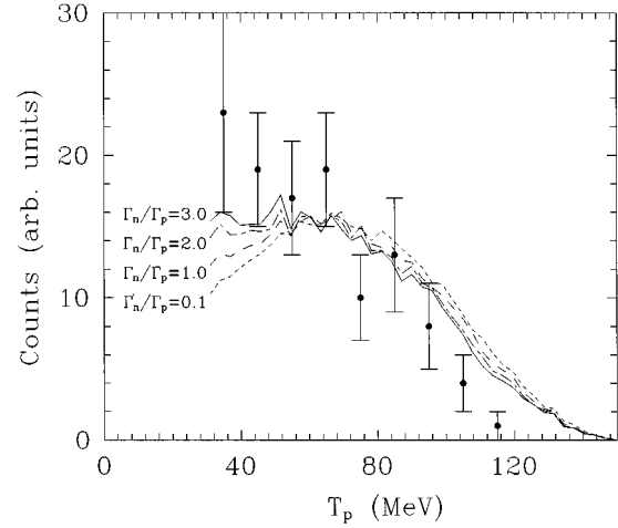
FIG. 16. Same as Fig. 15 but comparing with the experimental points of Ref. [5].
