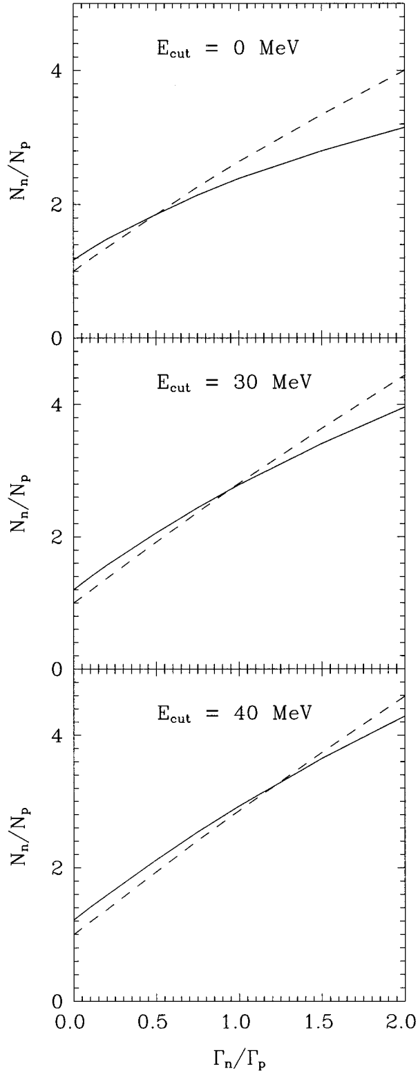
FIG. 11. N_n/N_p as a function of \Gamma_n/\Gamma_p in the decay of ^{12}_{\Lambda}\text{C} including final state interaction effects and applying energy cuts of 0, 30, and 40 MeV. Dashed line: 1N -induced mechanism. Solid line: (1N+2N) -induced mechanisms.
