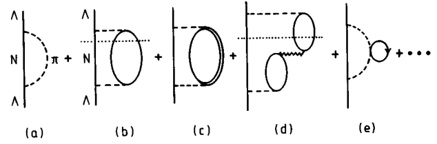
FIG. 1. \Lambda self-energy diagrams for the one-nucleon-induced channel from Refs. [13,15]. The dotted line cuts the states which are placed on shell in the evaluation of \text{Im}\Sigma .
