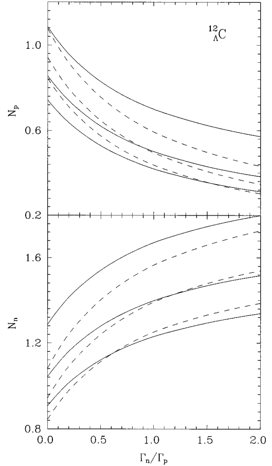
FIG. 12. Number of protons ( N_p ) and neutrons ( N_n ) per \Lambda decay event in ^{12}_{\Lambda}\text{C} as functions of \Gamma_n/\Gamma_p . Dashed lines: 1N -induced mechanism. Solid lines: (1N+2N) -induced mechanism. Final state interactions are considered and, from top to bottom, the results include energy cuts of 0, 30, and 40 MeV, respectively.
