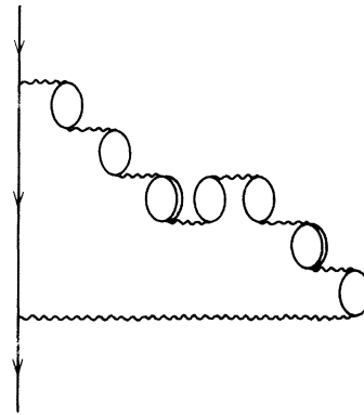
FIG. 2. Model for the nucleon self-energy. The wavy lines refer to \pi and \rho exchange plus additional short range correlations. The \pi and \rho are allowed to interact with the medium via p-h or \Delta -h excitation.
