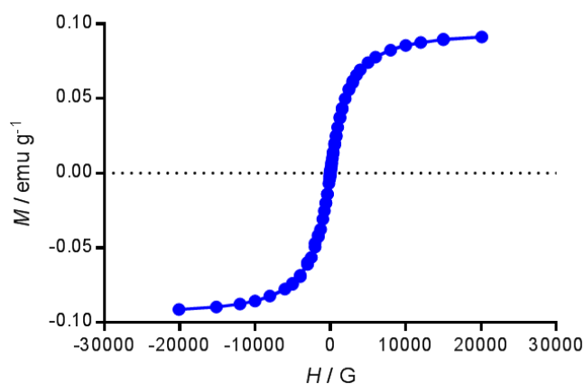
Figure 3. Mass magnetization as a function of the external magnet field for magnetic particles coated with oleic acid at 300 K. The external magnetic field was swept from 20,000 to −20,000 G and then back to 20,000 G.
