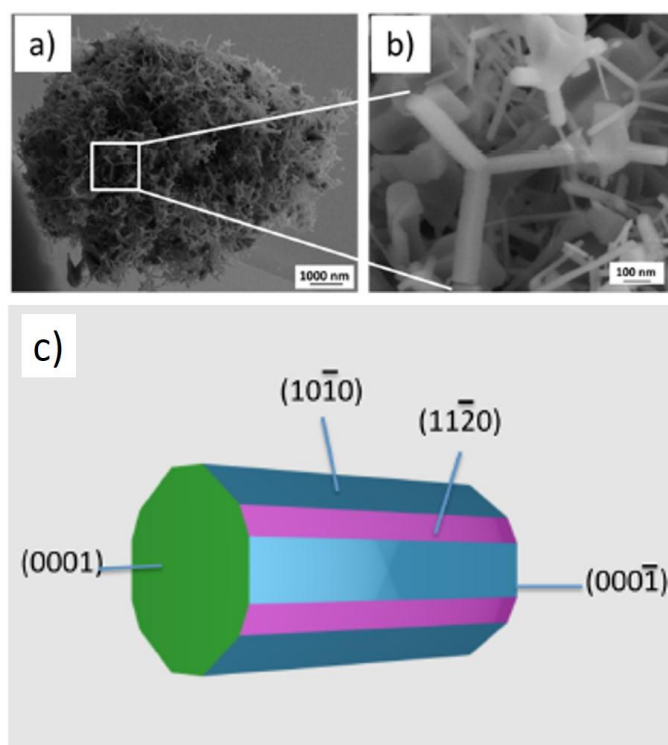
Fig. 1 Scanning electron microscope images of ZnO smoke: a) an ensemble of nanoparticles and b) a closer view of tetrapods and sticks present in the powder; and c) Wulff construction of ZnO stick derived from calculated surface energies, 39 following Wulff shape construction, 58 as previously described. 59
