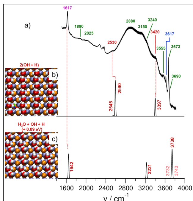
Fig. 5 Comparison between the a) IR spectrum recorded on ZnO smoke at RT after exposure to P_{\text{H}_2\text{O}} = 1 mbar - representative of the spectra shown in Fig. 2 - and calculated spectra associated to \text{H}_2\text{O} adlayer structures determined by DFT approach for ZnO( 11\bar{2}0 ) surface and representative structures: b) (2 \times 1)_{\text{fully-dissoc}} c) (2 \times 1)_{\text{half-dissoc}} . Blue and green highlighted frequencies correspond to ZnO( 000\bar{1} )-O and ZnO( 10\bar{1}0 ) orientation, respectively. The same colour code as in Figs. 3 and 4, is used for spheres representative of atoms. The deformation frequency ( 1617 \text{ cm}^{-1} ) of the water molecule is highlighted in violet.
