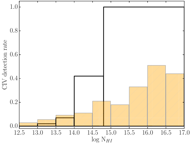
Figure 9. Detection rate of C IV absorbers (down to our detection limit of \log N_{\text{CIV}} = 11.4 ) as a function of the column density of the associated H I line (white, open histogram). The overplotted hatched histogram is the fraction of H I systems that arise within |\Delta v| < 300 \text{ km s}^{-1} and D_{\text{tran}} < 300 physical kpc from LB galaxies (adapted from Rudie et al. 2012).
