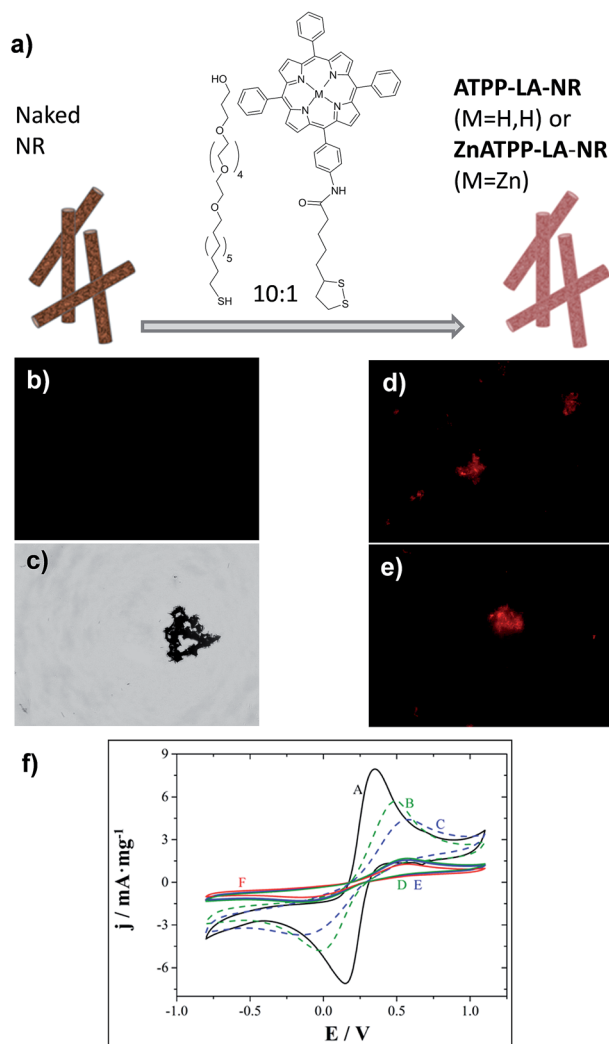
Fig. 5 Schematic representation of the NR functionalization with either ATTP-LA or ZnATTP-LA (a); fluorescence microscope images showing a mesh of non-functionalized naked NR (b) and the corresponding image with visible light (c); fluorescence microscope images showing a mesh of porphyrin-functionalized ATTP-LA-NR (d) and ZnATTP-LA-NR (e), identified by the red color. Magnification 400 \times ; Electrochemical probe of Fe(II)/Fe(III) system at 100 mV s -1 (f) showing curves for non-functionalized naked NR (A), NR-H (B), NR-Zn (C), ATTP-LA-NR (D), ZnATTP-LA-NR (E) and PEG-NR (F).
