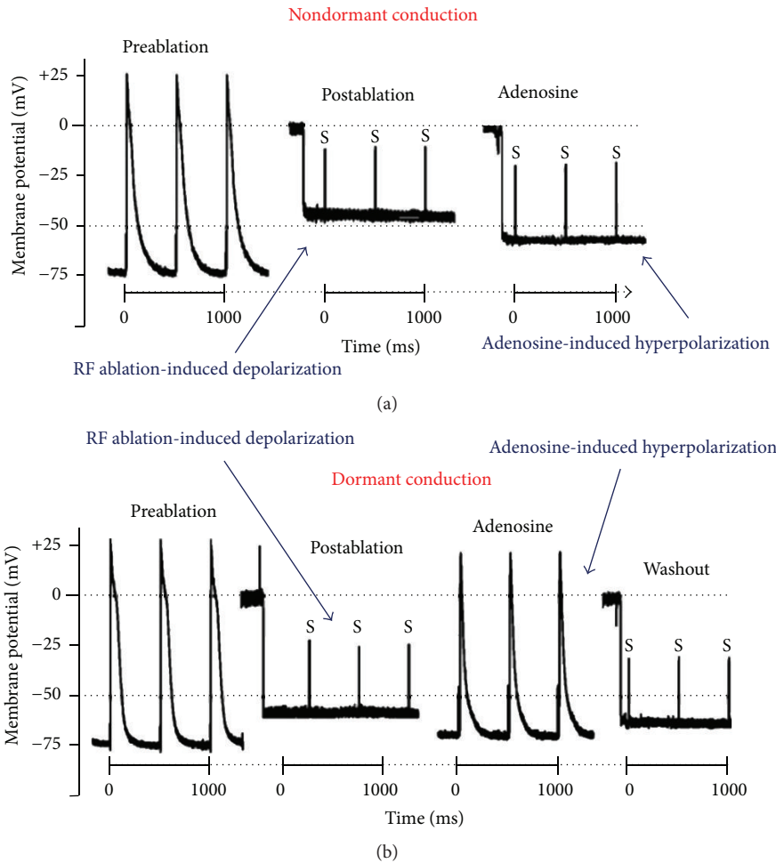
FIGURE 1: Microelectrode recordings before and after pulmonary vein isolation in a PV without dormant conduction (upper panel) and in a PV with dormant conduction (lower panel). S: stimulus artifacts with no response. Dotted line: excitability threshold at -50 mV (adapted from Datino et al. [7]).
