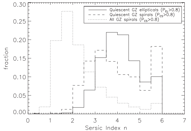
Figure 4. Sérsic index distribution of quiescent elliptical, quiescent spiral and all spiral galaxies in the DR7 spectroscopic catalogue. Only galaxies with debiased probability P_{\text{debiased}} > 0.8 are selected in all three cases. Quiescent spiral galaxies show a distribution closer to that of early types than that of ‘normal’ spirals.
