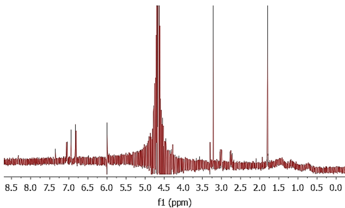
Figure S4.1: ^1\text{H} NMR spectrum of N -acetyldityrosine (NAdT) in \text{D}_2\text{O} .
