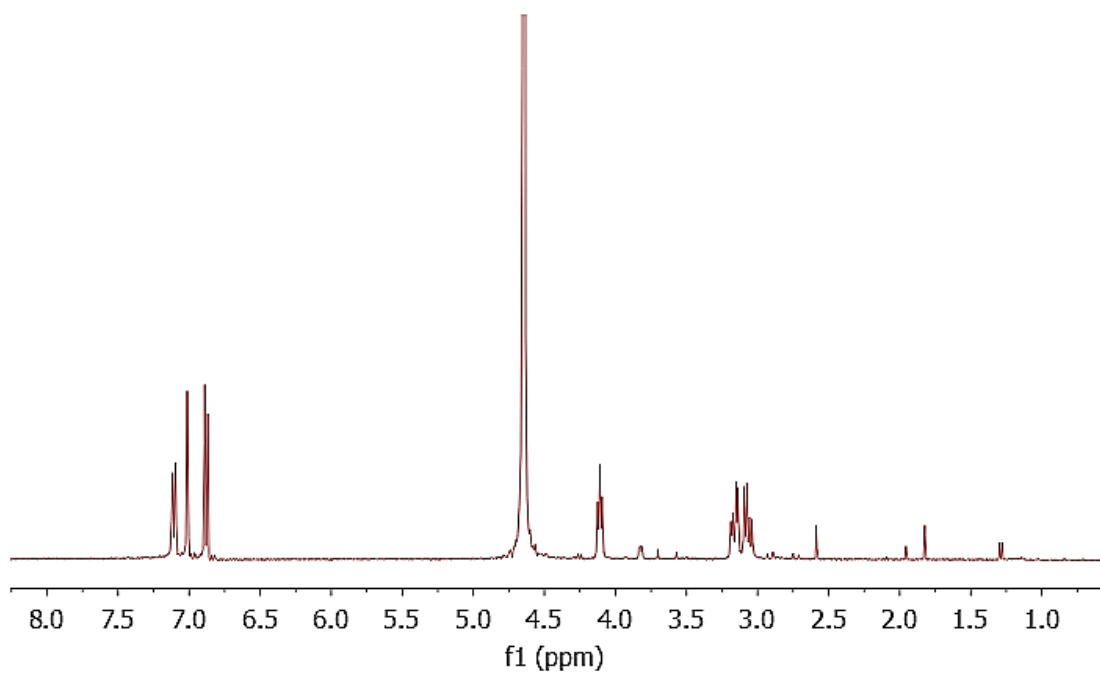
Figure S4.2: ^1\text{H} NMR spectrum of dityrosine in \text{D}_2\text{O} .
