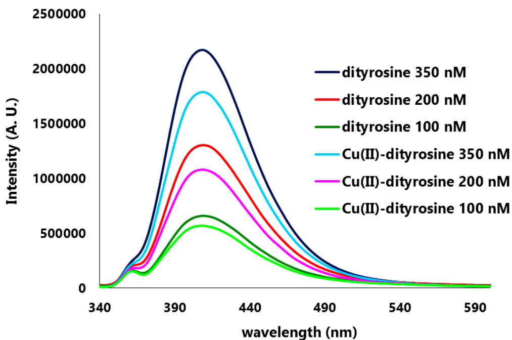
Figure S4.6: Fluorescence spectra of dityrosine in the presence and absence of equimolar amounts of \text{CuCl}_2 at concentrations 100, 200 or 350 nM in 100 mM HEPES (pH 7.4). \lambda_{\text{exc}} = 320 nm.
