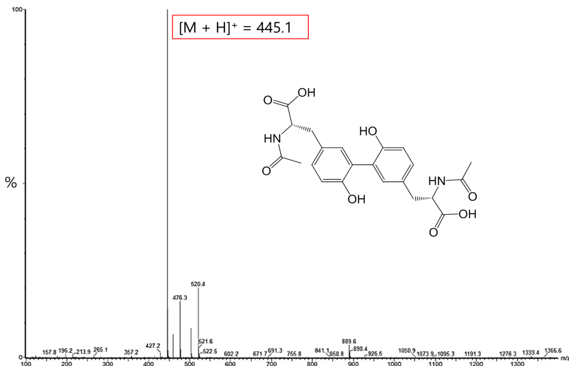
Figure S4.3: ESI mass spectrum of N -acetyldityrosine (NADT).
