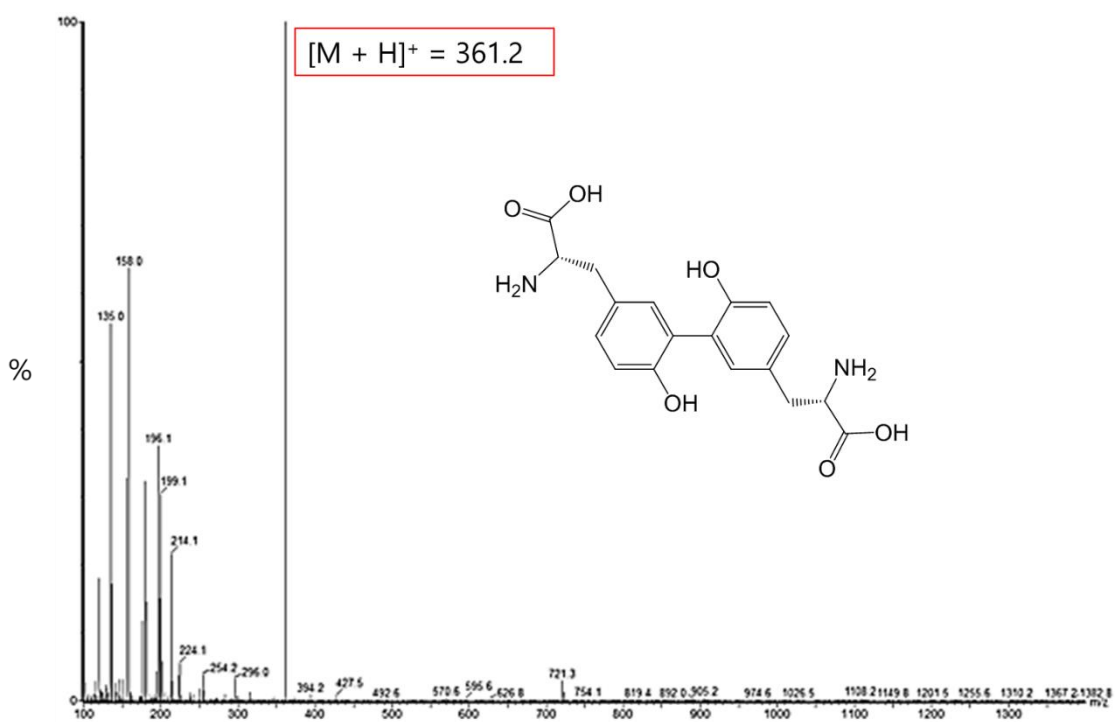
Figure S4.4: ESI mass spectrum of dityrosine.
