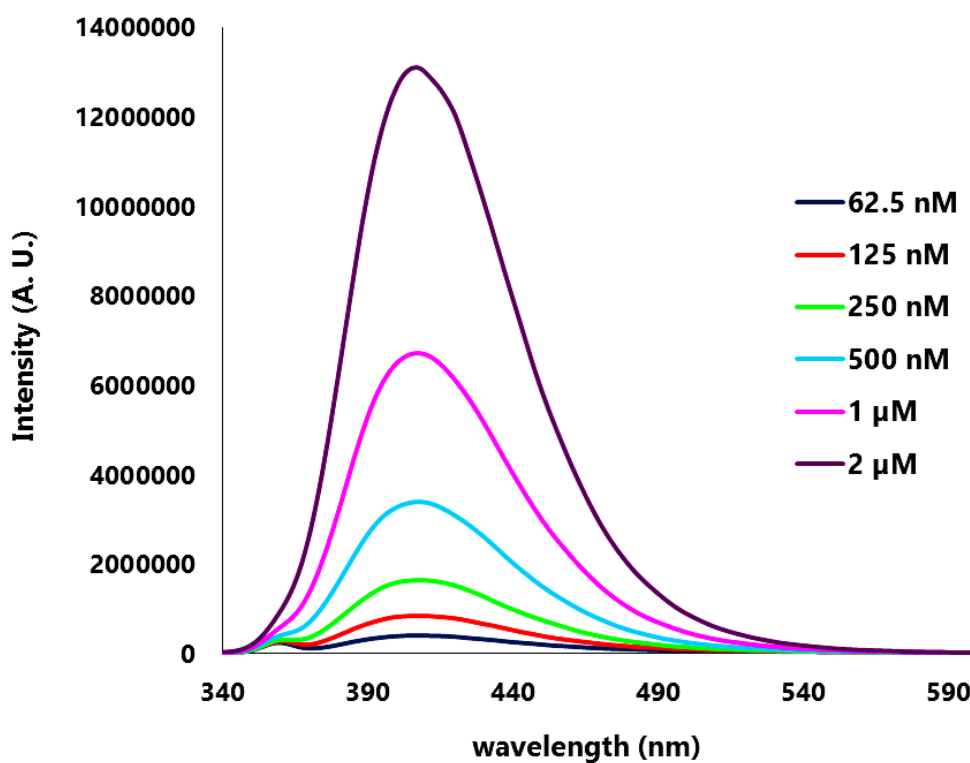
Figure S4.5: Fluorescence spectra of dityrosine at concentrations 62.5 nM-2 μM in 100 mM HEPES (pH 7.4). \lambda_{\text{exc}} = 320 nm.
