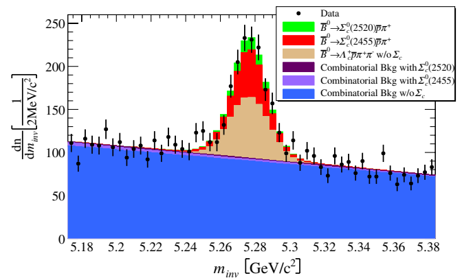
FIG. 5 (color online). Result of the fit to the m_{\text{inv}}:m_{\pm\pm} plane projected onto the m_{\text{inv}} axis. The data are shown as points with error bars; the fitted signal and background PDFs are overlaid as stacked histograms.
