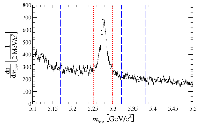
FIG. 1 (color online). Distribution of the invariant mass m_{\text{inv}}(\Lambda_c^+ \bar{p}\pi^+\pi^-) for events with m_{\text{ES}} in the region [5.272, 5.285] \text{ GeV}/c^2 . The red dotted lines indicate the signal region and the blue dashed lines the sideband regions. Higher multiplicity modes, such as B \rightarrow \Lambda_c^+ \bar{p}\pi^+\pi^-\pi , appear for m_{\text{inv}} < 5.14 \text{ GeV}/c^2 .
