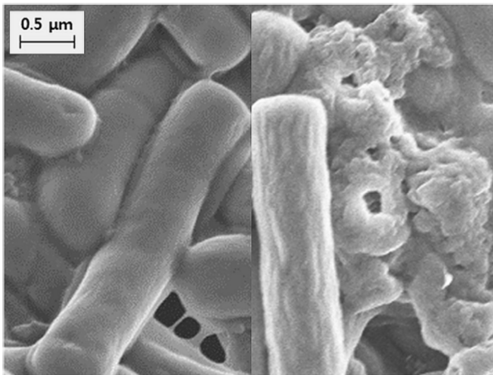
Figure 2. Comparison with non-treated (left panel) and tyndallized L. rhamnosus (right panel) [85].
