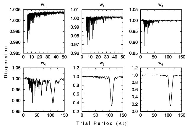
Figure 9. WPDm output for each wavelet plane of the data at the top of Fig. 6.
