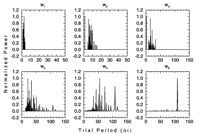
Figure 10. WCLEAN output for each wavelet plane of the data at the top of Fig. 6.
