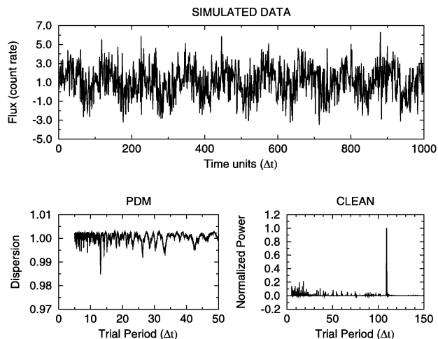
Figure 6. Top: simulated data of a Gaussian with 13.13-unit period, a FWHM of 6.0 units, amplitude = 0.5 and \sigma_{\text{noise}} = 1.5 , superimposed on the sinusoid with 108.5-unit period and amplitude = 1.0. Bottom: PDM and CLEAN outputs of this data set.
