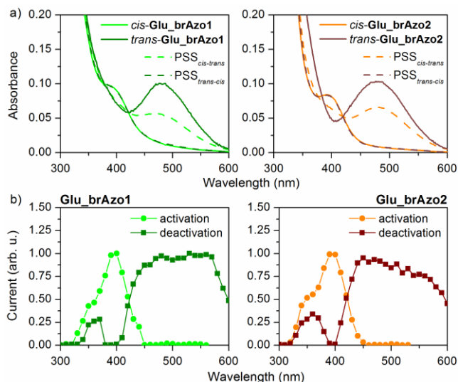
Figure 3. (a) Absorption spectra of both isomers of Glu_brAzo1 and Glu_brAzo2 in PBS:DMSO 1:1, as well as of the PSS mixtures obtained under cis-trans (λ exc = 405 nm) and trans-cis (λ exc = 532 nm) photoisomerization. (b) Activation and deactivation spectra of GluK2 in HEK293 cells after perfusion of Glu_brAzo1 or Glu_brAzo2 and irradiation to induce cis-trans (for activation) and trans-cis (for deactivation) photoisomerization.
