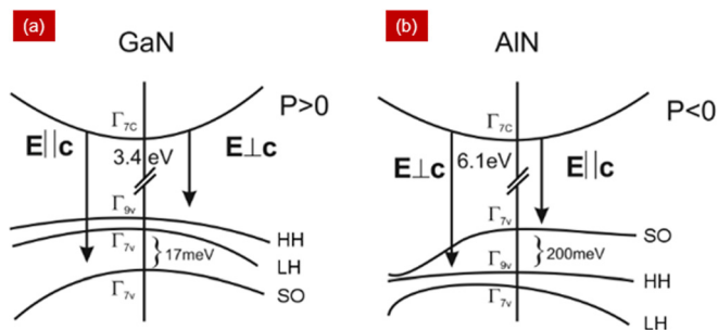
FIG. 6. Conduction band and valence band sequence in (a) GaN and (b) AlN, indicating a change of polarization. From Rass and Lobo-Ploch, III-Nitride Ultraviolet Emitters . Copyright 2016 Springer Nature. Reprinted with permission from Springer Nature. 113
