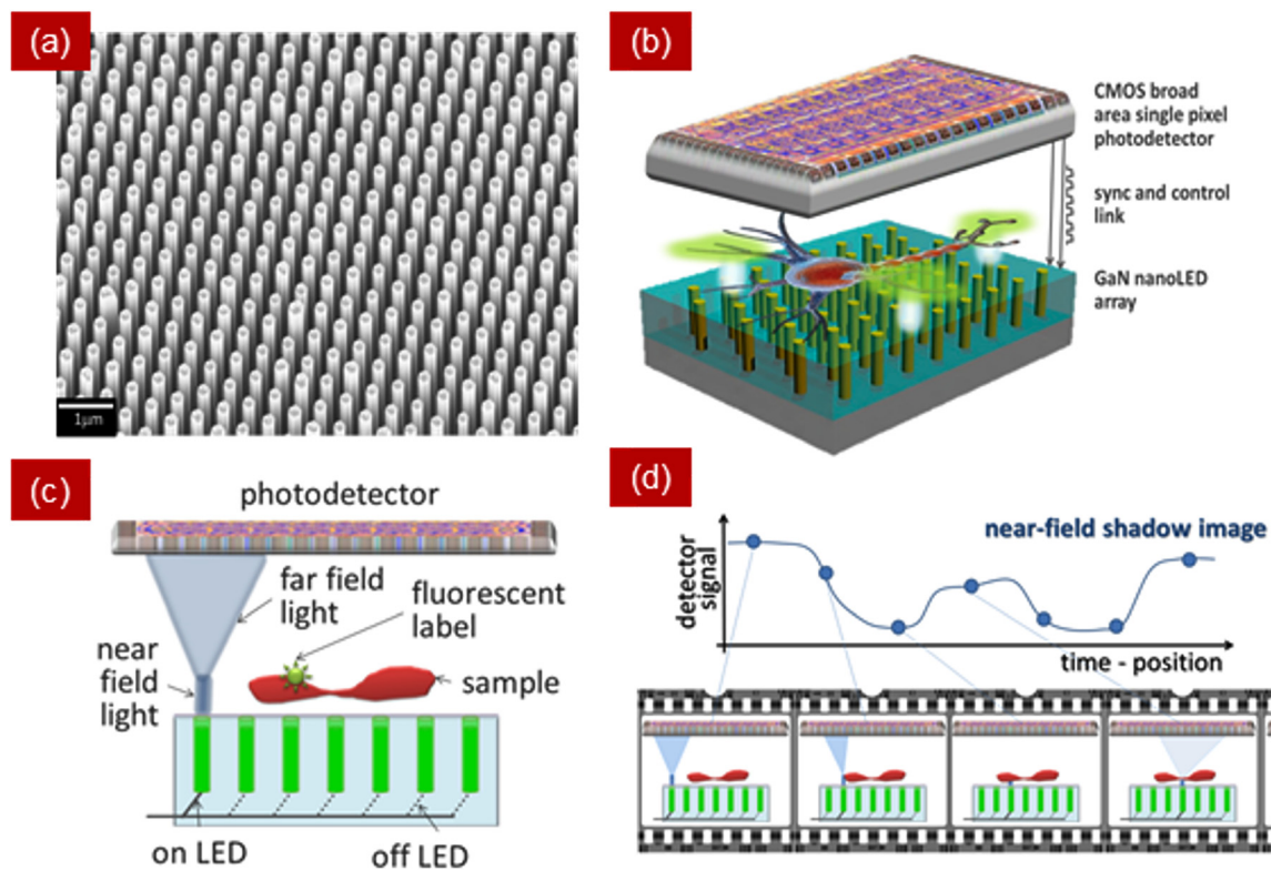
FIG. 10. (a) Array of InGaN 3D nano-LEDs. Each one of the nanorods contains one fully functional LED element, which can be activated as an independent point light source. Current technology makes it feasible achieving pitches between nano-LEDs of a few hundred nanometers. This means that independent point light sources with a spacing below the wavelength of the emitted light are at reach. (b) One possible application of this extremely dense nano-LED array is direct optical microscopy, without lenses, in combination with a broad area light detector, located in front and close to the nano-LED array. (c) and (d) Such a system can produce direct shadow images, by scanning the sample with one nano-LED pixel after the other, and monitoring the intensity through the sample, which means approaching the typical wavelengths of the light emitted. This approach opens the door to a new kind of highly miniaturized, high resolution microscope.
