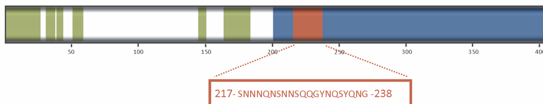
Figure 2. PrionW predictions of prion-like domains (PrLDs) and amyloid cores in the sequences of the genuine yeast prions New1, Ure2 and Rnq1. Folded domains, disordered regions, predicted PrLDs and amyloid cores are shown in white, green, blue and red, respectively.
