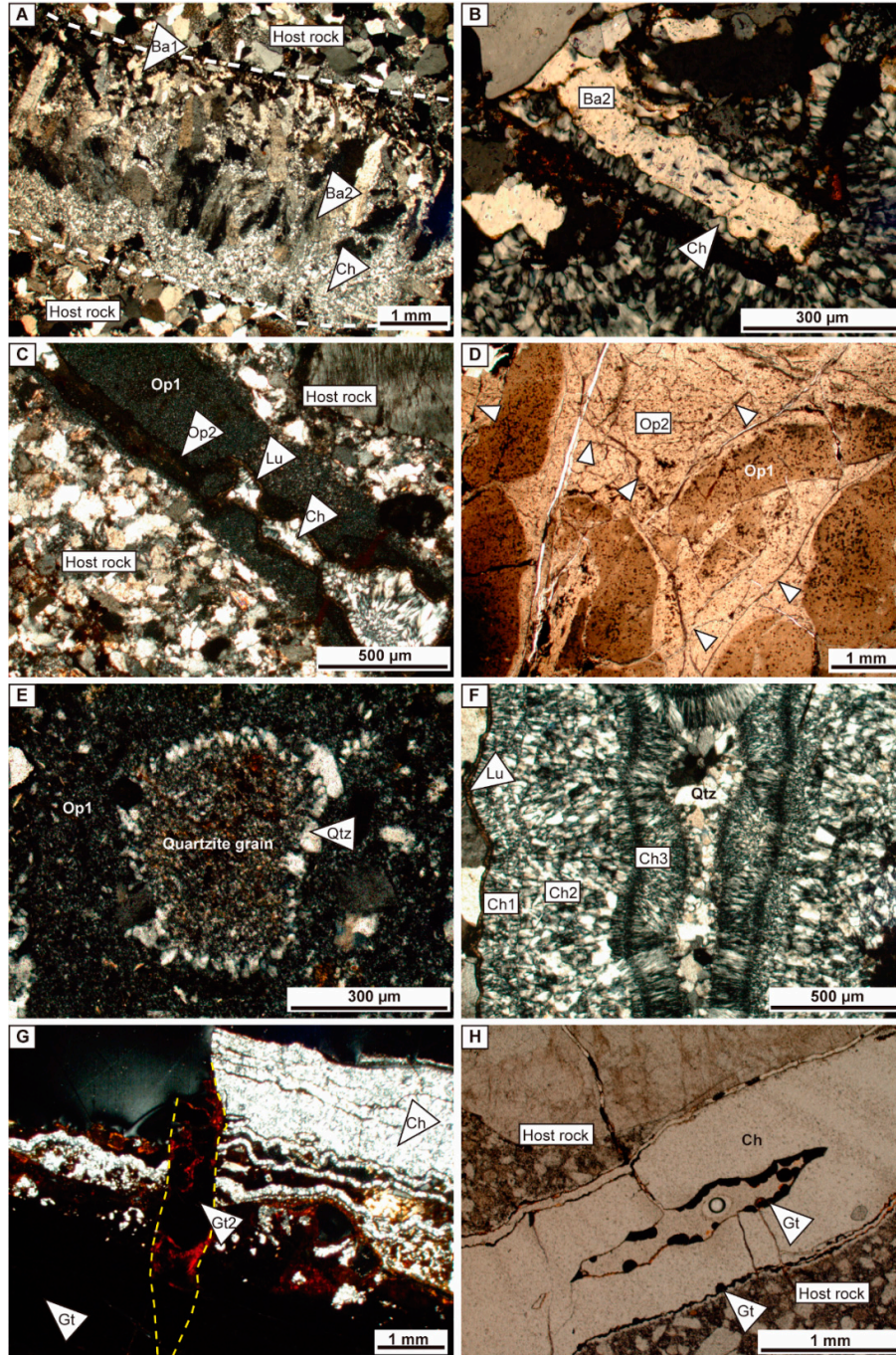
Figure 5. Cements in the fractures in the silicified area of the Castell Unit. (A) Fracture cemented by two generations of barite (Ba1 and Ba2) and a later generation of chalcidony (Ch) (XPL). Fracture walls are marked with a white dashed-line. (B) Detail of the replacement of barite (Ba2) by chalcidony (Ch) (XPL). (C) Silica varieties cementing a fracture according to their purity and crystallinity: two opal generations (Op1 and Op2), lussatite (Lu) and chalcidony (Ch) (XPL). (D) Fracture filled by two generations of opal affected by millimeter-scale cracks (white arrows). (E) Quartzite clast contained in a fracture cemented by opal that has developed a quartz rim (Qtz). (F) Fracture cemented by the silica sequence, lussatite, three generations of chalcidony and quartz (XPL). (G) Fracture filled by goethite (Gt) (and minor barite), alternation of goethite and chalcidony and finally pure chalcidony. The sequence is later cut by a fracture (yellow dashed- line) cemented by iron oxides (Gt2) (XPL). (H) Fracture cemented by several episodes of chalcidony and later goethite botryoids (PPL).
