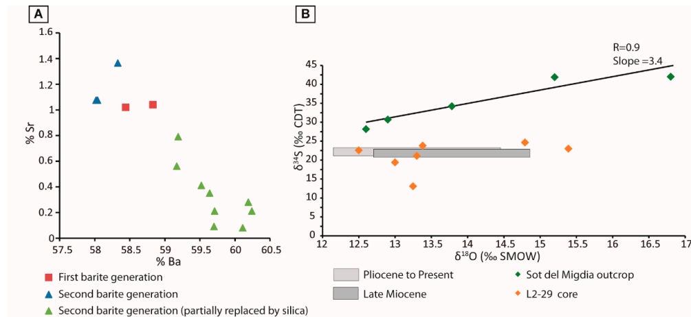
Figure 7. (A) Barite compositions plotted in a %Sr vs %Ba binary diagram. (B) \delta^{34}\text{S} vs \delta^{18}\text{O} binary diagram. Grey boxes represent the isotopic composition of seawater for the Late Miocene and from Pliocene to present according to [57].
