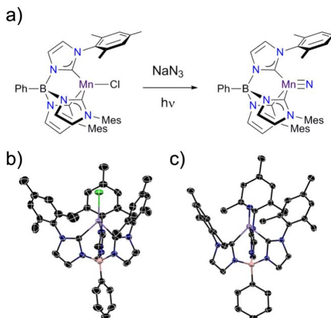
Figure 2. (a) Synthesis of PhB(MesIm) 3 Mn≡N ( 2 ) and X-ray crystal structures of (b) PhB(MesIm) 3 Mn IV -Cl ( 1 ), and (c) PhB(MesIm) 3 Mn V ≡N ( 2 ) with thermal ellipsoids shown at 50 % probability; H atoms are omitted for clarity. Black, blue, lilac, pink and green ellipsoids represent C, N, Mn, B and Cl atoms, respectively.
