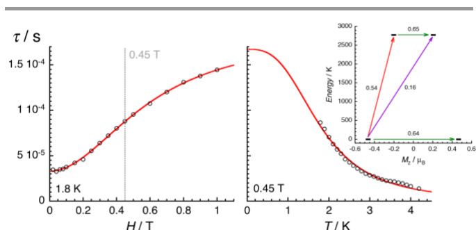
Figure 9. Field (left, at 1.8 K) and temperature (right, at 0.45 T) dependences of the average relaxation time for 2 estimated from the Figures 6 and 7. The red lines are the best fit obtained with the theoretical approach developed in the text. Inset: Lowest two Kramers doublets and ab initio computed relaxation mechanism with the MOLCAS code (CASSCF+RASSI level). The thick black lines are Kramers doublets shown as a function of their magnetic moment, M_z , along the main anisotropy axis ( z ). The green arrows correspond to the quantum tunnelling mechanism (QTM) of ground and first excited states while purple arrow shows the hypothetical Orbach relaxation process. The red arrow indicates the transition between the ground and first KDs. The values close to the arrows indicate the matrix elements of the transition magnetic moments (above 0.1, an efficient spin relaxation mechanism is expected). Thus, this figure highlights that the QTM through the Kramers doublet ground state is dominating the relaxation process at low temperatures.
