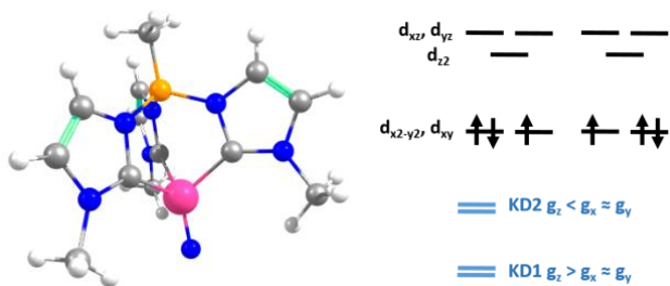
Figure 8. Left: Model complex for 2 used in the electronic structure calculations. Color code: Mn (magenta); N (blue); C (gray); B (orange); H (white). Right, top: main orbital configurations contributing to the ground state. Right, bottom: relation between components of the g tensor of the first two Kramers' doublets (KD1 and KD2).
