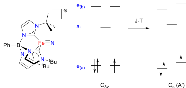
Figure 1. Effect of the Jahn-Teller distortion on the d-orbital splitting in a four-coordinate Fe(V) nitride complex.
