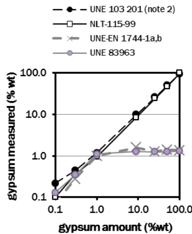
fig 2. Gypsum content (in %wt) determined according to the different norms, of the seven synthetic samples with known gypsum content.
