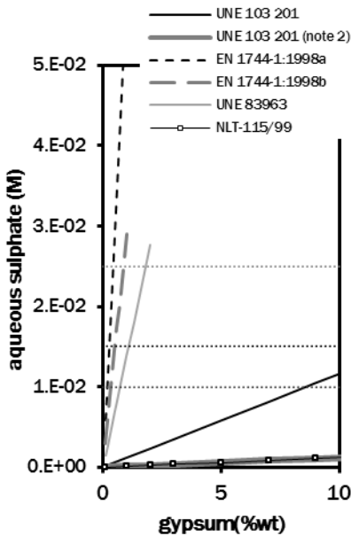
fig 1. Concentration of aqueous sulphate that would enter in solution for different gypsum contents if saturation is not considered. Dotted lines show the range of aqueous sulphate concentration in equilibrium with gypsum according to r.1.
