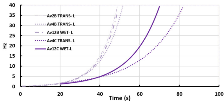
Figure 10. Curves for Equation (14) for TRANS avalanches with values in Table 2 of the SON section of the spectrograms for sites B and C, respectively. Curves of avalanche Av12 WET-L are included in the plot because the curvatures at sites B and C are similar to those of the TRANS avalanches. Notice that this avalanche does not meet our requirements. The classification corresponds to that in Table 1. The curves were shifted in time for comparison. Capital letters B and C are added to the avalanche name in accordance with the site.
