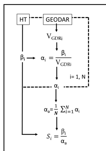
Figure 12. Diagram of the procedure for obtaining the speed values S_i and the attenuation parameter \alpha_a from the \beta_i values obtained from HT and the V_{GDRi} derived from the GEODAR images. The value of \alpha_e is obtained similarly omitting the powder snow avalanches, and avalanches Av11C TRANS-L and Av12C WET-L.
