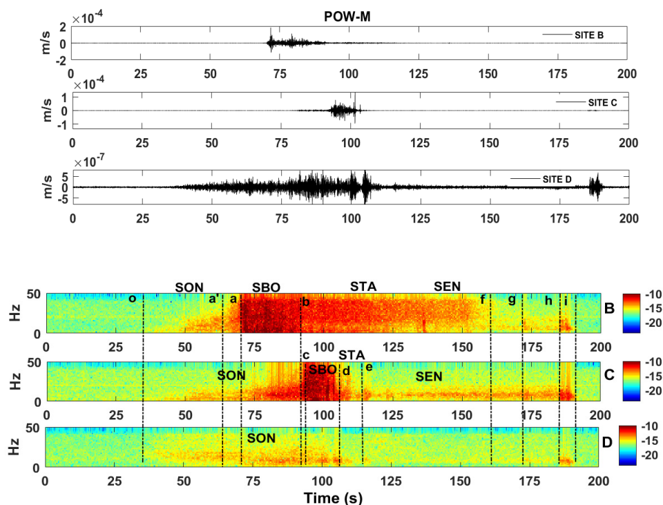
Figure 3. Time series (top) and spectrograms (bottom) of the final seismogram (FS) of the POW avalanche recorded at sites B, C, and D (Figures 1 and 2) displayed with a common time in s (horizontal axis). Vertical axis in time series corresponds to the ground movement generated by the avalanche in m/s. Vertical axis in the spectrograms corresponds to frequency in Hz. Spectrogram amplitudes (in color) in 10^{-1} dB. The sections Signal ONset (SON), Signal Body (SBO), STA, and SEN of each spectrogram indicate characteristics of the avalanche. Explanation of the details are included in Appendix B.
