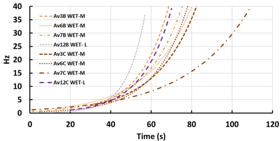
Figure 11. Curves for Equation (14) for WET avalanches with values in Table 2 of the SON section of the spectrograms for sites B and C, respectively. Observe the different behavior of the curves of Av12 WET-L that does not meet our requirements. The classification corresponds to that in Table 1. The curves were shifted in time for comparison. Capital letters B and C are added to the avalanche name in accordance with the site.
