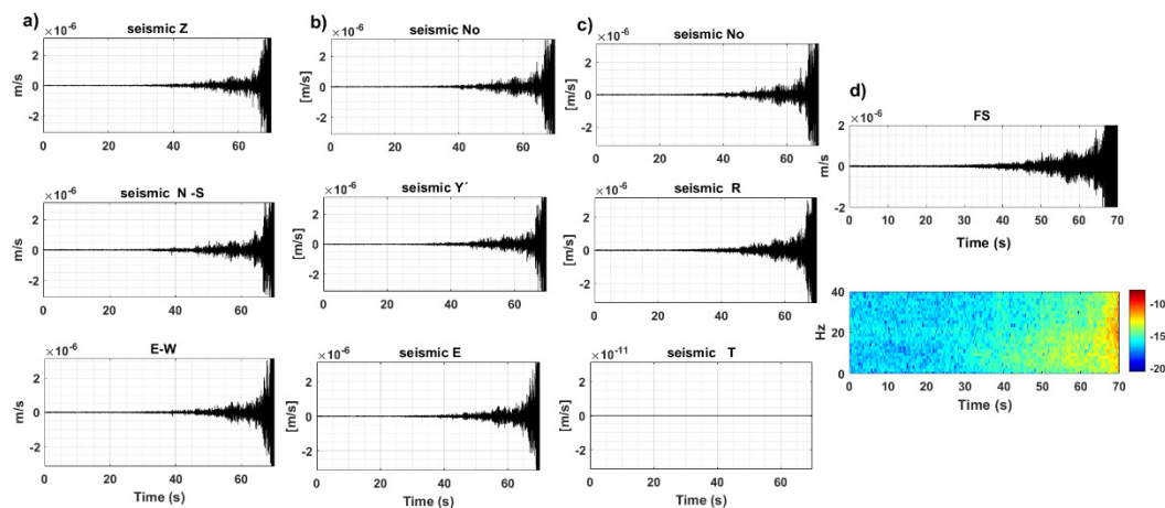
Figure A2. Example of the result of the application of the rotations to the SON section of an avalanche. (a) Time series the original seismic components (Z, N-S, E-W). (b) Time series after application of R1(\phi) in (No, Y' and E-W components). (c) Time series after application of R2(\xi(t)) in No, R, and T components. (d) Time series (up) and spectrogram (down) of FS, result of the representation in polar coordinates. Vertical axis in the time series ground movement in m/s. Horizontal axis time in s. Spectrogram amplitudes (in color) in 10^{-1} dB.
