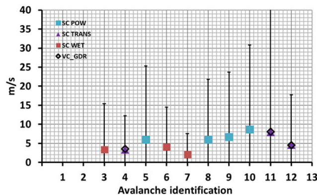
Figure 15. Estimates of the avalanche front speeds for site C according to their type. Error bars are included. Values of SC for the 3 types of avalanches correspond to columns SC_a in Table 3. VC\_GDR are the velocities V_{GDR} derived from GEODAR measurements for site C. The speed values for POW avalanches are plotted although no data from GEODAR velocities are shown given that the comparison is meaningless (see text for explanation).
