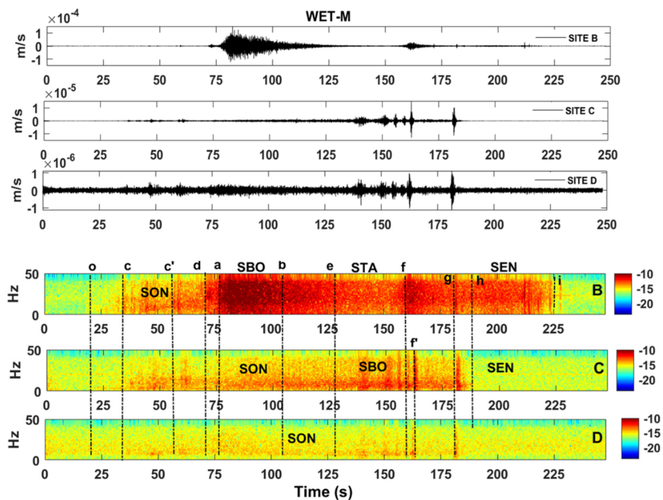
Figure 5. Time series (top) and spectrograms (bottom) of the final seismogram (FS) of the WET avalanche recorded at sites B, C, and D (Figures 1 and 2) displayed with a common time in s (horizontal axis). Vertical axis in time series corresponds to the ground movement generated by the avalanche in m/s. Vertical axis in the spectrograms corresponds to frequency in Hz. Spectrogram amplitudes (in color) in 10^{-1} dB. The sections SON, SBO, STA, and SEN of each spectrogram indicate characteristics of the avalanche. Explanation of the details are included in Appendix B.
