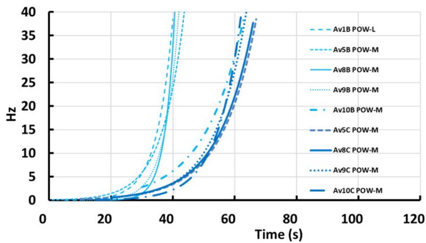
Figure 9. Curves of Equation (14) for POW avalanches with values in Table 2 in the SON section of the spectrograms for sites B and C, respectively. The classification corresponds to that in Table 1. The curves were shifted in time for comparison. Capital letters B and C are added to the avalanche name in accordance with the site. Observe the different behavior of the curve of av10B POW-M that does not meet our requirements.
