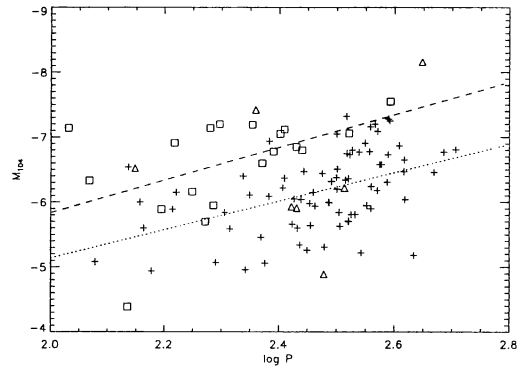
Figure 2. Period–luminosity relations in 104 filter. Crosses represent Miras belonging to group 1, triangles to group 2 and squares to group 3. Dotted line and dashed line are the period–luminosity fit relations for group 1 and 3 respectively.
