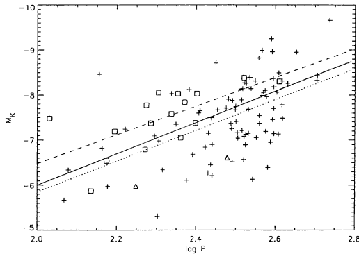
Figure 1. Period–luminosity relations in K band. Crosses represent Miras belonging to group 1, triangles to group 2 and squares to group 3. Dotted line and dashed line are the period–luminosity fit relations for group 1 and 3 respectively. Solid line is the period–luminosity relation determined by van Leeuwen et al. (1997).
