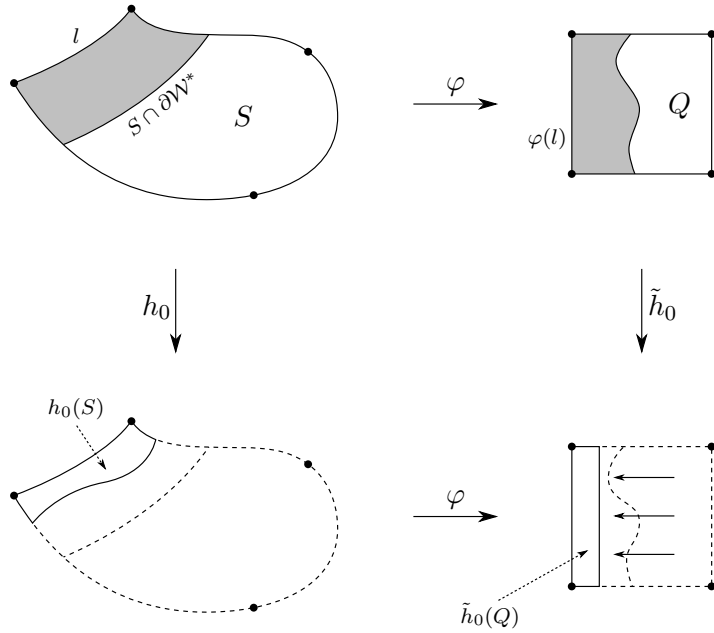
Figure 8: For the construction of the map h: \widehat{\mathbb{C}} \rightarrow \widehat{\mathbb{C}} , we first define an auxiliary map h_0: S \rightarrow h_0(S) as a conjugation of a quasi-conformal map on Q , where it is easy to define the desired local dynamics. In grey we find S \cap \mathcal{W}^* (and its \varphi -image), the subset where we want h_0(S) to end up.
