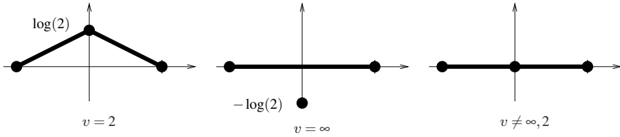
Figure 2. Local roof functions in Example 6.2.
