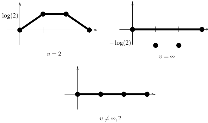
Figure 3. Local roof functions in Example 6.2.
